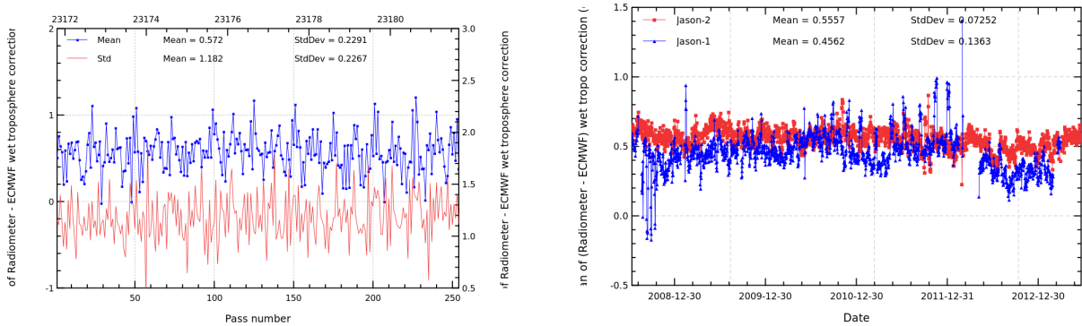
FIGURE 11 – Pass monitoring of wet troposphere differences between radiometer and ECMWF model for Jason-2 cycle 182 (left) and daily monitoring of wet troposphere differences between radiometer and ECMWF model (right).
