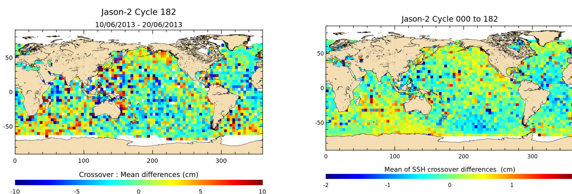
FIGURE 12 – Mean SSH at crossovers for cycle 182 (left) and over the whole Jason-2 period (right).
