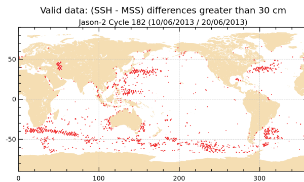
FIGURE 18 – Differences higher than a 30 cm threshold for cycle 182.
