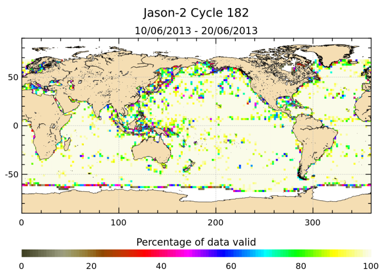
FIGURE 3 – Percentage of valid measurements for cycle 182.
