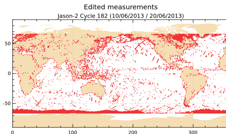
FIGURE 2 – Edited measurements for cycle 182.
