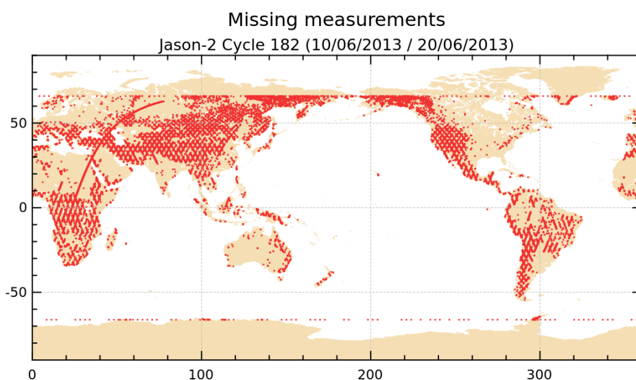
FIGURE 1 – Missing measurements for cycle 182.
