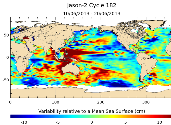
FIGURE 17 – Sea level anomaly relative to MSS for cycle 182.
