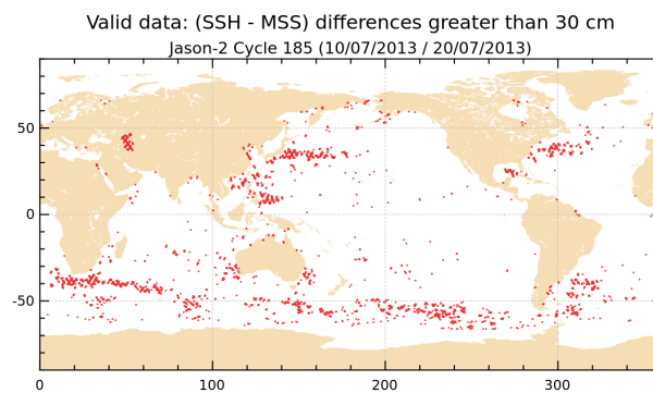
FIGURE 18 – Differences higher than a 30 cm threshold for cycle 185.
