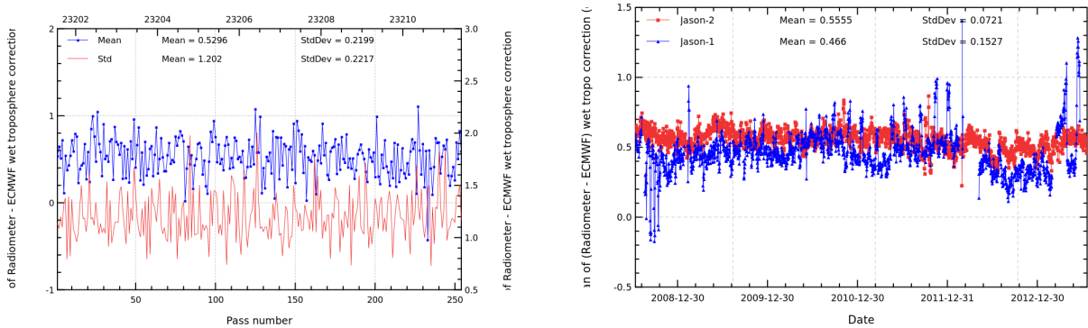
FIGURE 11 – Pass monitoring of wet troposphere differences between radiometer and ECMWF model for Jason-2 cycle 185 (left) and daily monitoring of wet troposphere differences between radiometer and ECMWF model (right).
