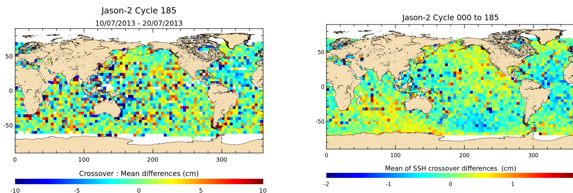
FIGURE 12 – Mean SSH at crossovers for cycle 185 (left) and over the whole Jason-2 period (right).
