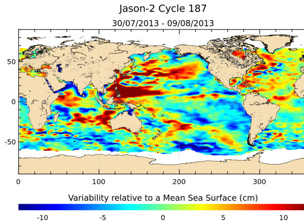
FIGURE 17 – Sea level anomaly relative to MSS for cycle 187.
