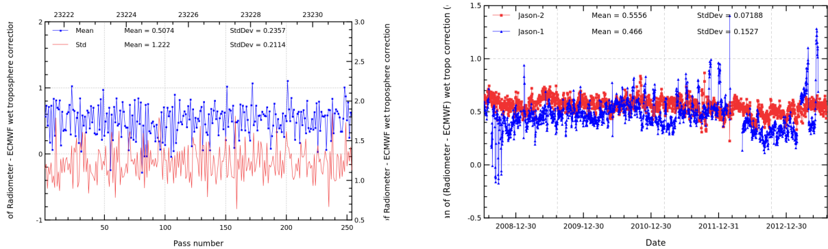
FIGURE 11 – Pass monitoring of wet troposphere differences between radiometer and ECMWF model for Jason-2 cycle 187 (left) and daily monitoring of wet troposphere differences between radiometer and ECMWF model (right).
