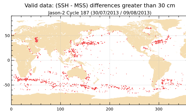
FIGURE 18 – Differences higher than a 30 cm threshold for cycle 187.
