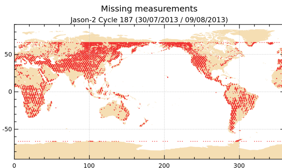
FIGURE 1 – Missing measurements for cycle 187.
