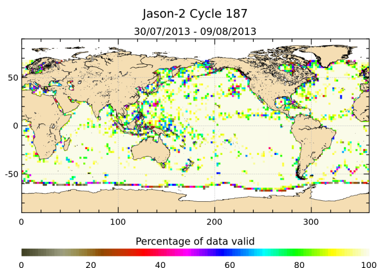
FIGURE 3 – Percentage of valid measurements for cycle 187.
