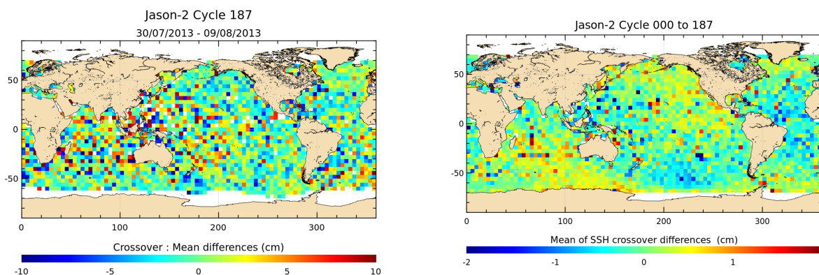
FIGURE 12 – Mean SSH at crossovers for cycle 187 (left) and over the whole Jason-2 period (right).
