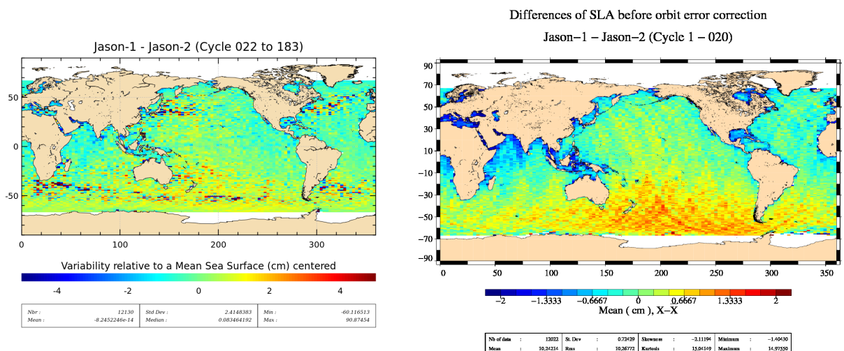
FIGURE 19 – Jason-1 – Jason-2 SLA differences averaged over whole Jason-2 period since cycle 022 until cycle 183 (left), and for flight formation phase (cycle 001 to 020) (right).
