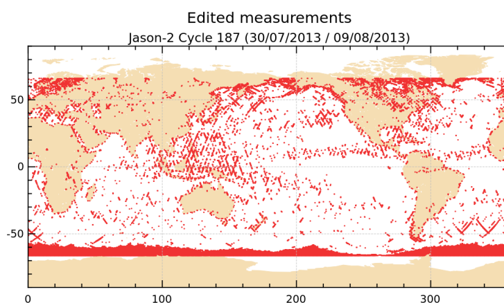
FIGURE 2 – Edited measurements for cycle 187.
