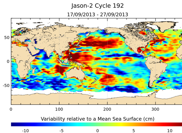
FIGURE 17 – Sea level anomaly relative to MSS for cycle 192.
