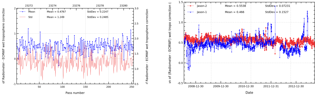
FIGURE 11 – Pass monitoring of wet troposphere differences between radiometer and ECMWF model for Jason-2 cycle 192 (left) and daily monitoring of wet troposphere differences between radiometer and ECMWF model (right).
