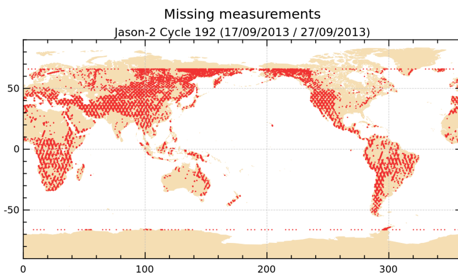
FIGURE 1 – Missing measurements for cycle 192.
