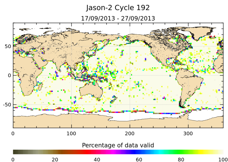
FIGURE 3 – Percentage of valid measurements for cycle 192.
