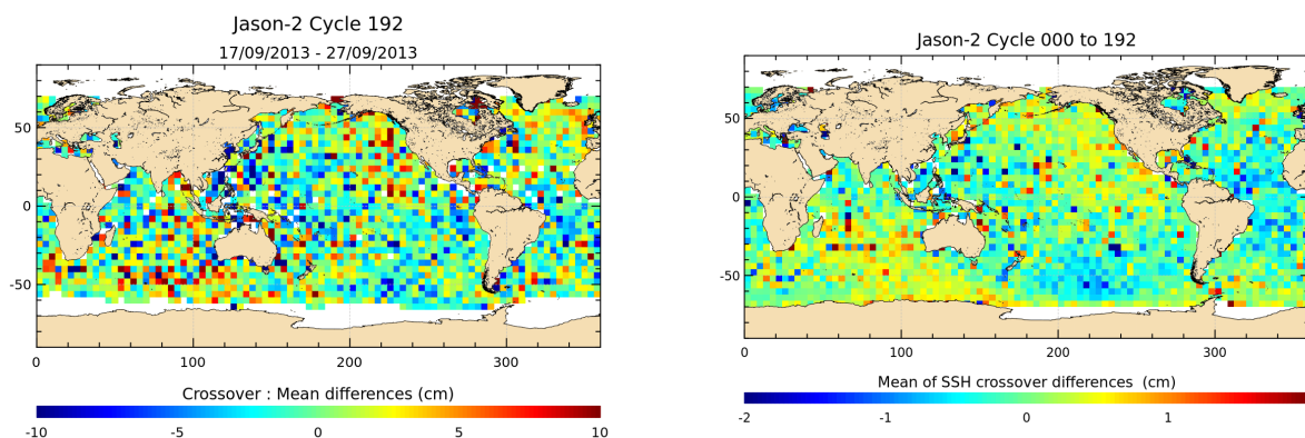
FIGURE 12 – Mean SSH at crossovers for cycle 192 (left) and over the whole Jason-2 period (right).
