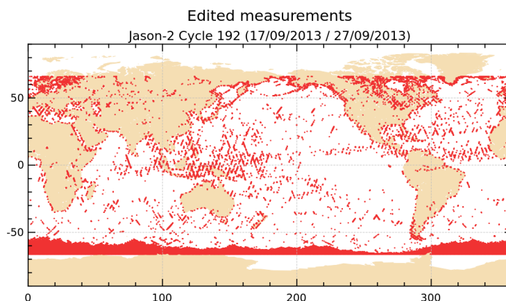
FIGURE 2 – Edited measurements for cycle 192.
