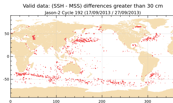
FIGURE 18 – Differences higher than a 30 cm threshold for cycle 192.
