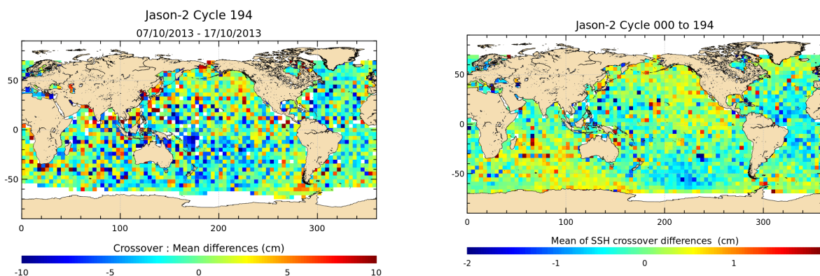
FIGURE 12 – Mean SSH at crossovers for cycle 194 (left) and over the whole Jason-2 period (right).
