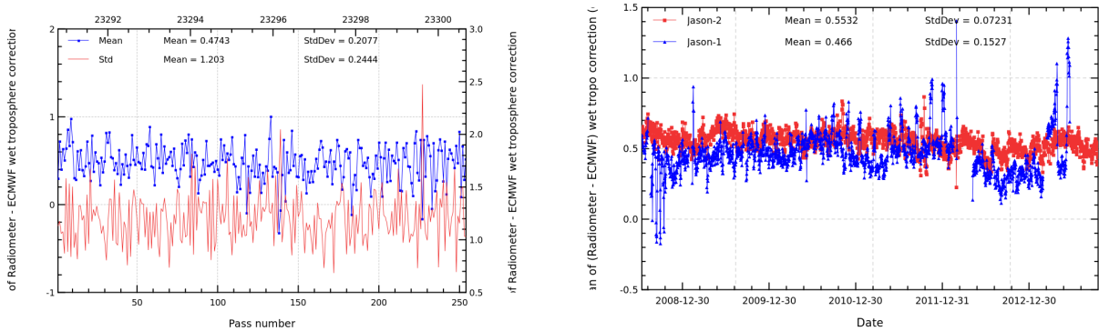
FIGURE 11 – Pass monitoring of wet troposphere differences between radiometer and ECMWF model for Jason-2 cycle 194 (left) and daily monitoring of wet troposphere differences between radiometer and ECMWF model (right).
