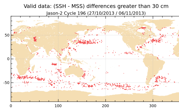
FIGURE 18 – Differences higher than a 30 cm threshold for cycle 196.
