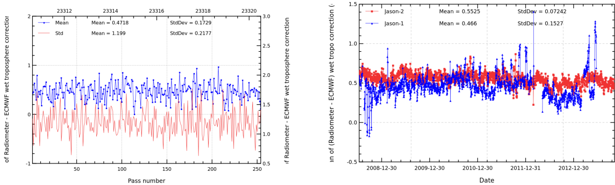
FIGURE 11 – Pass monitoring of wet troposphere differences between radiometer and ECMWF model for Jason-2 cycle 196 (left) and daily monitoring of wet troposphere differences between radiometer and ECMWF model (right).
