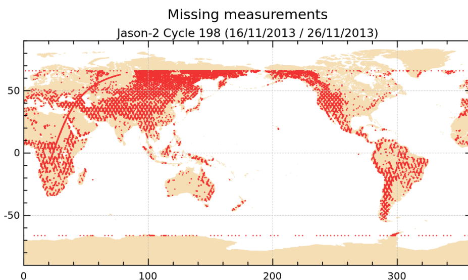
FIGURE 1 – Missing measurements for cycle 198.
