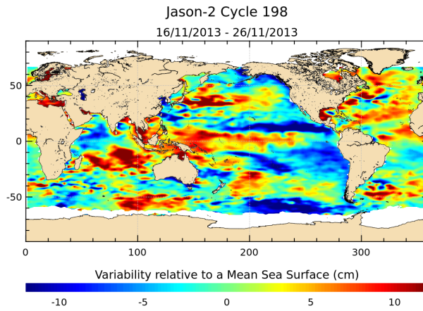
FIGURE 17 – Sea level anomaly relative to MSS for cycle 198.
