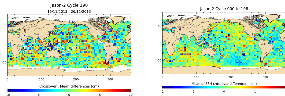
FIGURE 12 – Mean SSH at crossovers for cycle 198 (left) and over the whole Jason-2 period (right).
