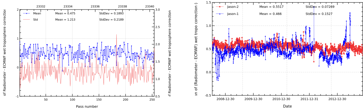
FIGURE 11 – Pass monitoring of wet troposphere differences between radiometer and ECMWF model for Jason-2 cycle 198 (left) and daily monitoring of wet troposphere differences between radiometer and ECMWF model (right).
