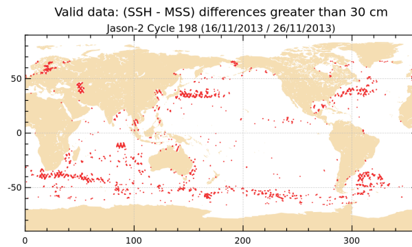
FIGURE 18 – Differences higher than a 30 cm threshold for cycle 198.
