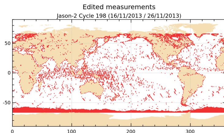
FIGURE 2 – Edited measurements for cycle 198.
