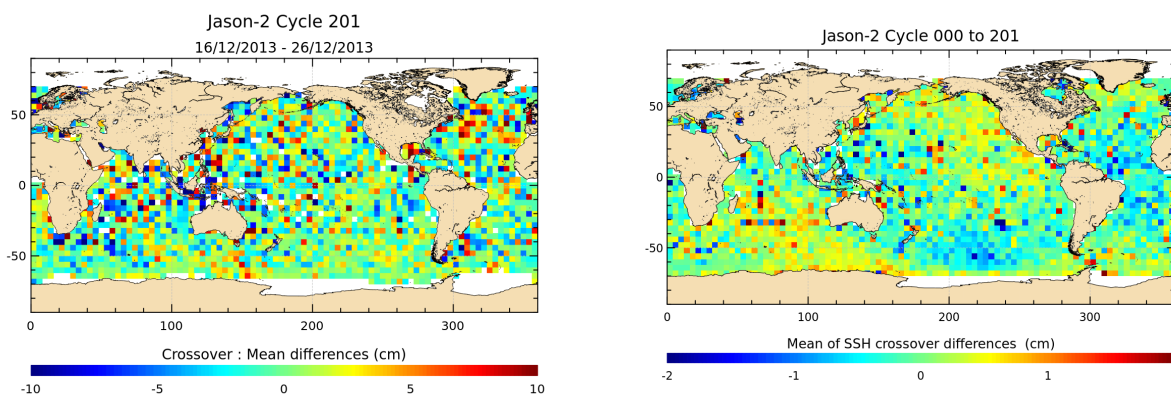
FIGURE 12 – Mean SSH at crossovers for cycle 201 (left) and over the whole Jason-2 period (right).
