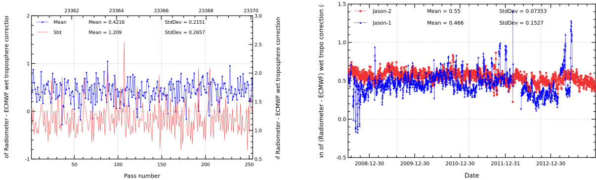
FIGURE 11 – Pass monitoring of wet troposphere differences between radiometer and ECMWF model for Jason-2 cycle 201 (left) and daily monitoring of wet troposphere differences between radiometer and ECMWF model (right).
