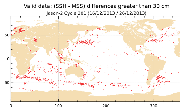
FIGURE 18 – Differences higher than a 30 cm threshold for cycle 201.
