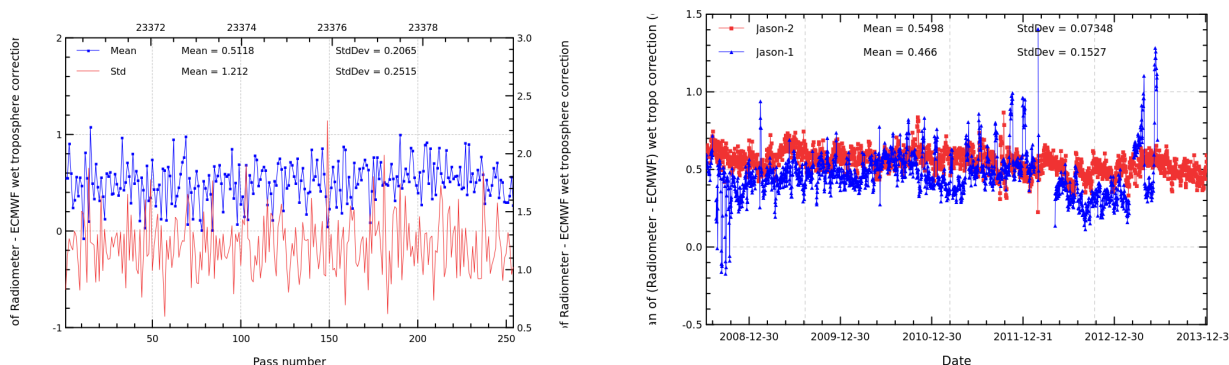
FIGURE 11 – Pass monitoring of wet troposphere differences between radiometer and ECMWF model for Jason-2 cycle 202 (left) and daily monitoring of wet troposphere differences between radiometer and ECMWF model (right).
