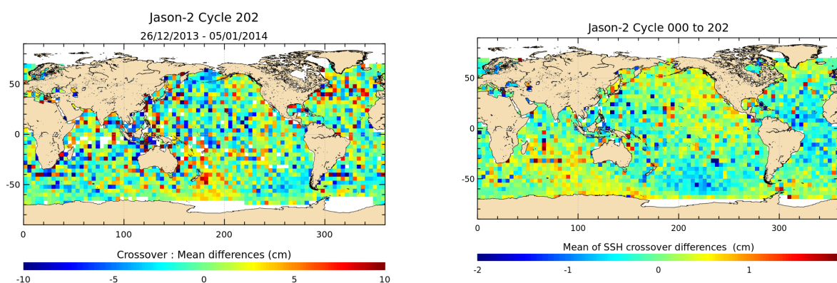
FIGURE 12 – Mean SSH at crossovers for cycle 202 (left) and over the whole Jason-2 period (right).
