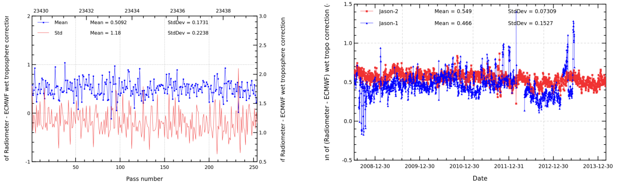
FIGURE 11 – Pass monitoring of wet troposphere differences between radiometer and ECMWF model for Jason-2 cycle 208 (left) and daily monitoring of wet troposphere differences between radiometer and ECMWF model (right).
