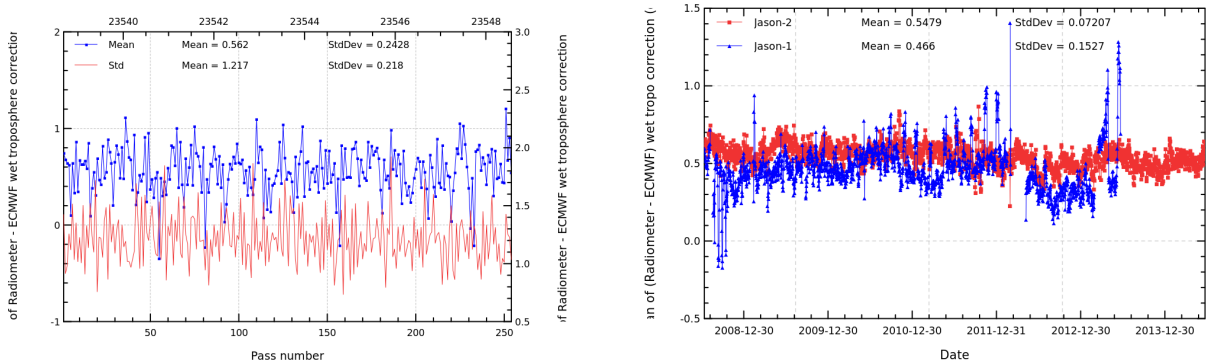
FIGURE 11 – Pass monitoring of wet troposphere differences between radiometer and ECMWF model for Jason-2 cycle 219 (left) and daily monitoring of wet troposphere differences between radiometer and ECMWF model (right).
