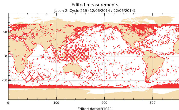
FIGURE 2 – Edited measurements for cycle 219.
