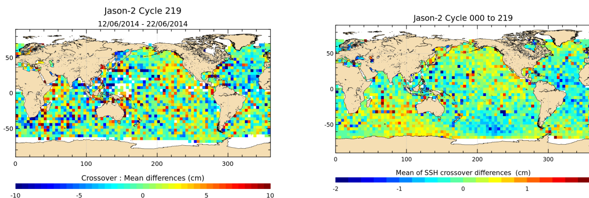
FIGURE 12 – Mean SSH at crossovers for cycle 219 (left) and over the whole Jason-2 period (right).
