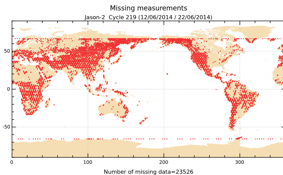
FIGURE 1 – Missing measurements for cycle 219.
