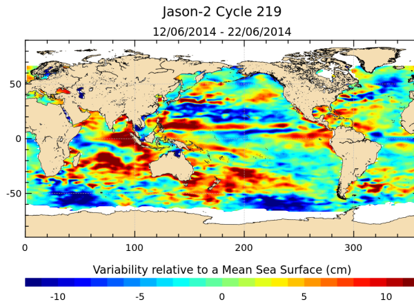
FIGURE 17 – Sea level anomaly relative to MSS for cycle 219.
