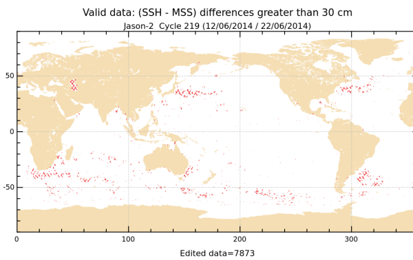
FIGURE 18 – Differences higher than a 30 cm threshold for cycle 219.
