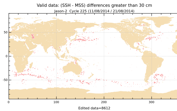
FIGURE 18 – Differences higher than a 30 cm threshold for cycle 225.
