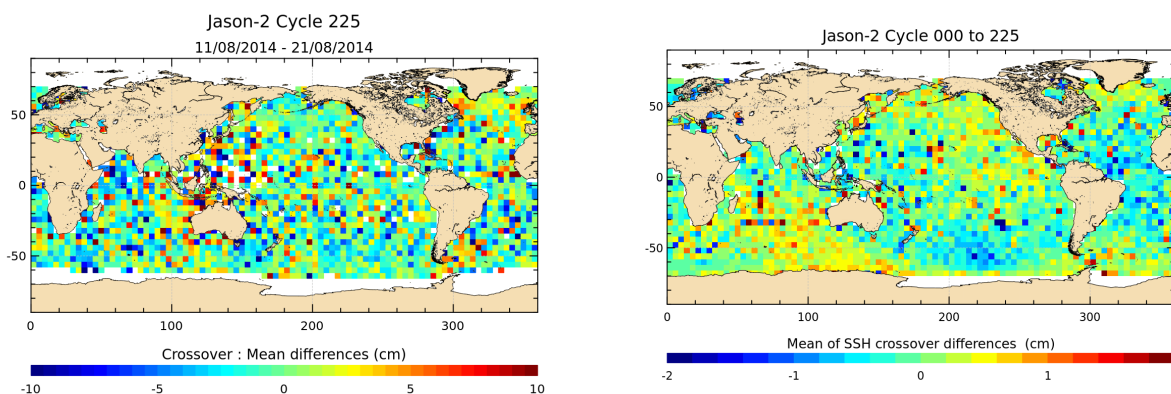
FIGURE 12 – Mean SSH at crossovers for cycle 225 (left) and over the whole Jason-2 period (right).
