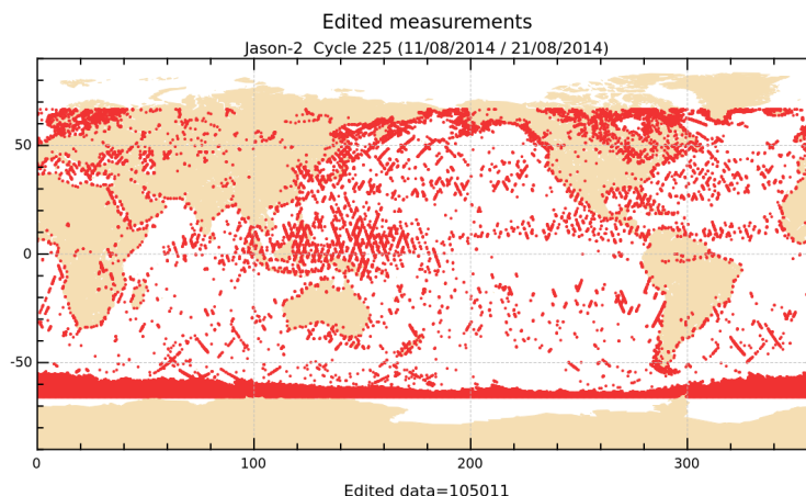
FIGURE 2 – Edited measurements for cycle 225.
