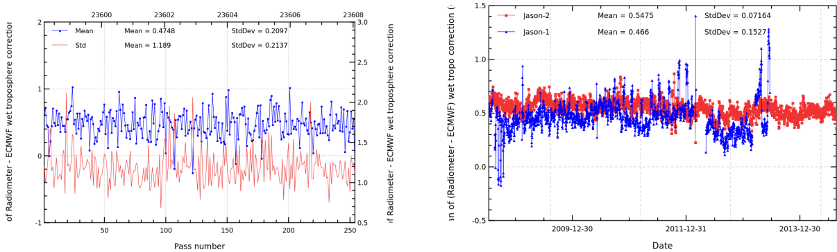
FIGURE 11 – Pass monitoring of wet troposphere differences between radiometer and ECMWF model for Jason-2 cycle 225 (left) and daily monitoring of wet troposphere differences between radiometer and ECMWF model (right).
