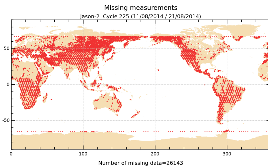
FIGURE 1 – Missing measurements for cycle 225.
