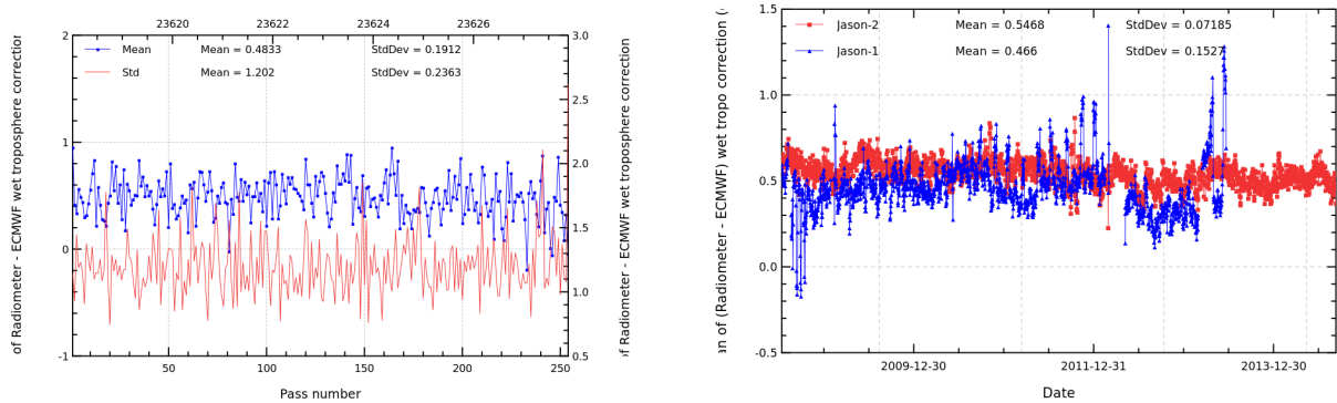
FIGURE 11 – Pass monitoring of wet troposphere differences between radiometer and ECMWF model for Jason-2 cycle 227 (left) and daily monitoring of wet troposphere differences between radiometer and ECMWF model (right).
