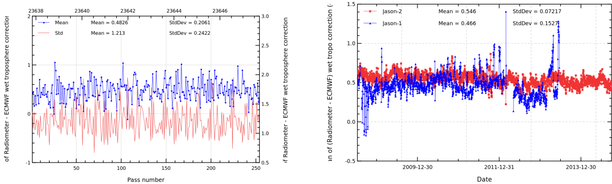
FIGURE 11 – Pass monitoring of wet troposphere differences between radiometer and ECMWF model for Jason-2 cycle 229 (left) and daily monitoring of wet troposphere differences between radiometer and ECMWF model (right).
