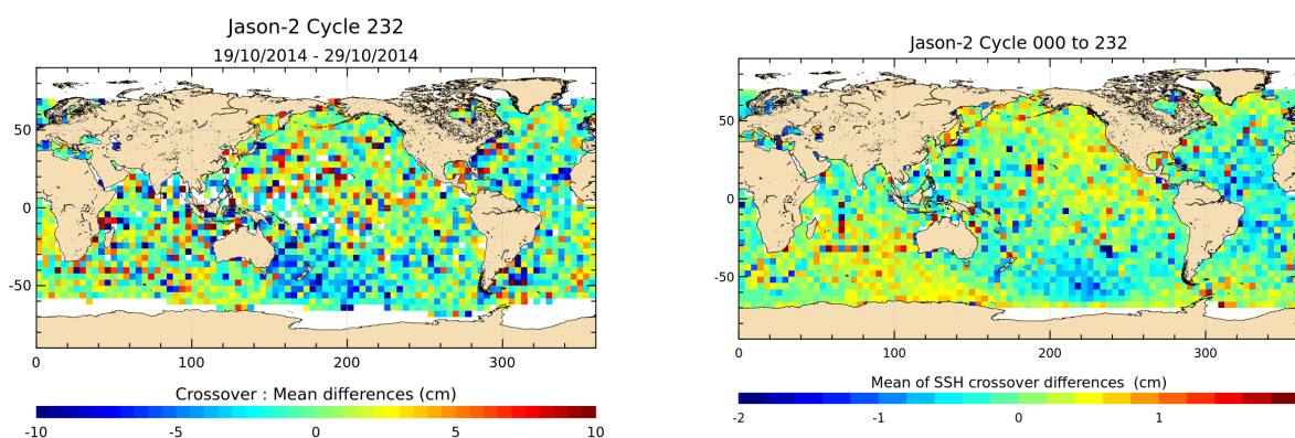
FIGURE 12 – Mean SSH at crossovers for cycle 232 (left) and over the whole Jason-2 period (right).
