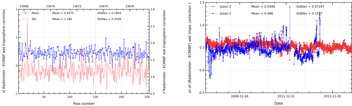
FIGURE 11 – Pass monitoring of wet troposphere differences between radiometer and ECMWF model for Jason-2 cycle 232 (left) and daily monitoring of wet troposphere differences between radiometer and ECMWF model (right).
