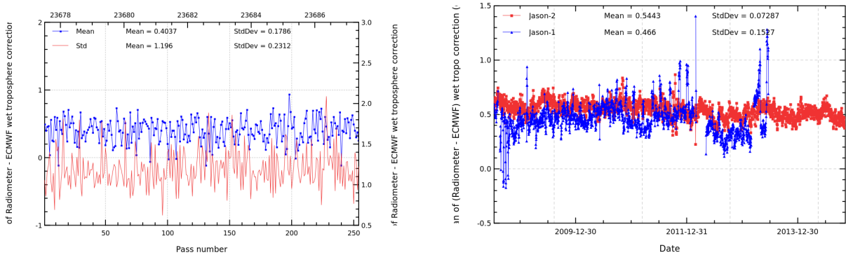
FIGURE 11 – Pass monitoring of wet troposphere differences between radiometer and ECMWF model for Jason-2 cycle 233 (left) and daily monitoring of wet troposphere differences between radiometer and ECMWF model (right).
