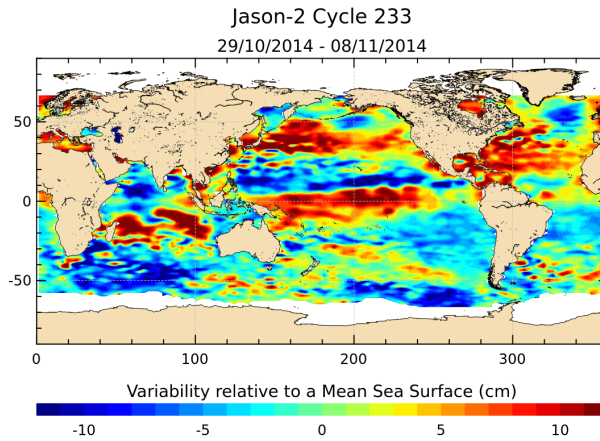
FIGURE 17 – Sea level anomaly relative to MSS for cycle 233.
