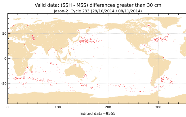
FIGURE 18 – Differences higher than a 30 cm threshold for cycle 233.
