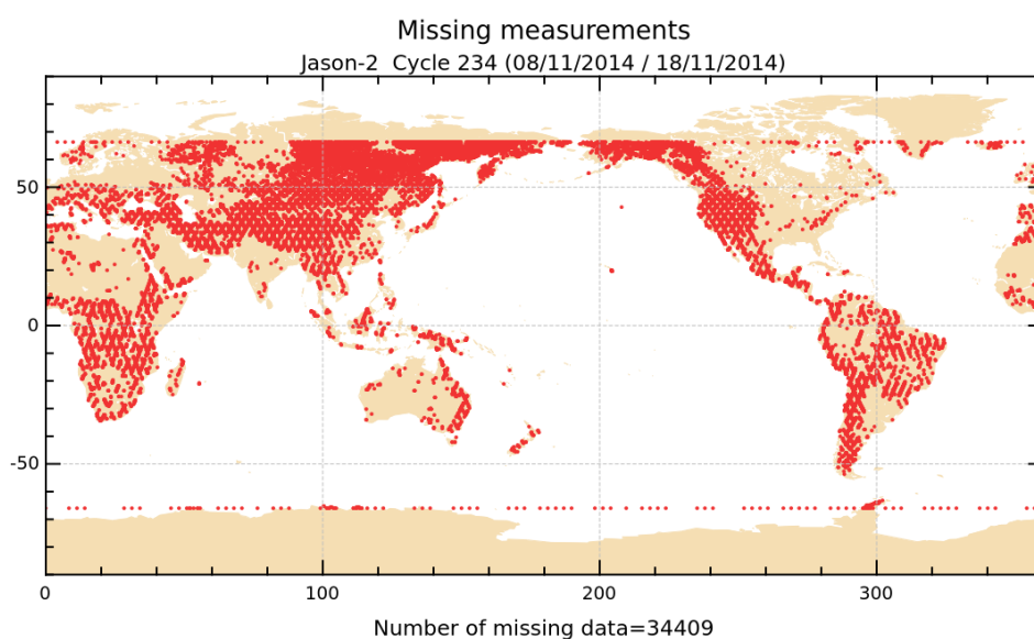
FIGURE 1 – Missing measurements for cycle 234.
