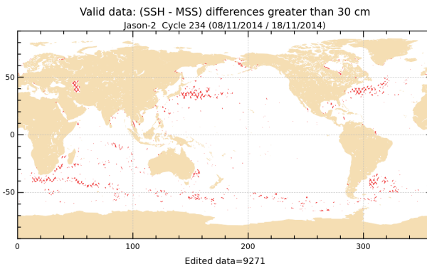
FIGURE 18 – Differences higher than a 30 cm threshold for cycle 234.
