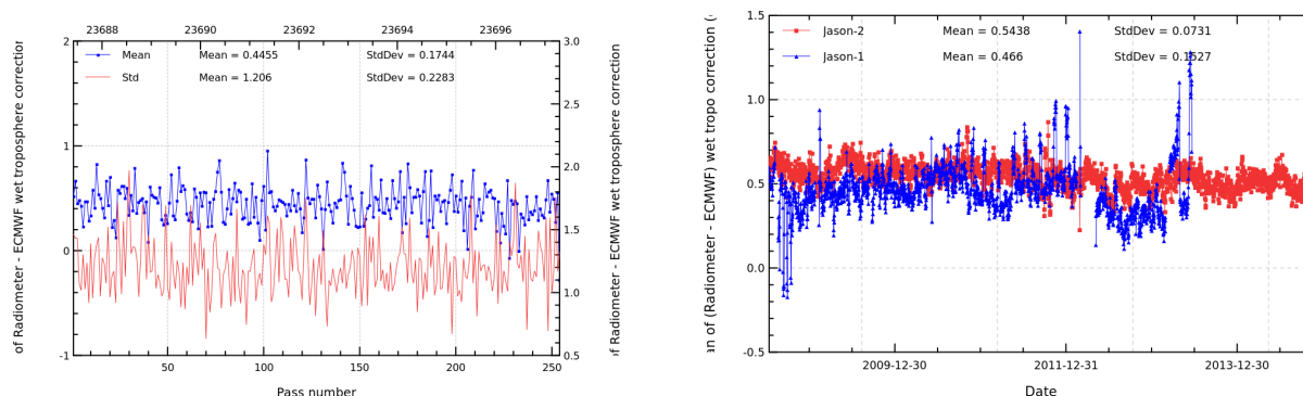
FIGURE 11 – Pass monitoring of wet troposphere differences between radiometer and ECMWF model for Jason-2 cycle 234 (left) and daily monitoring of wet troposphere differences between radiometer and ECMWF model (right).
