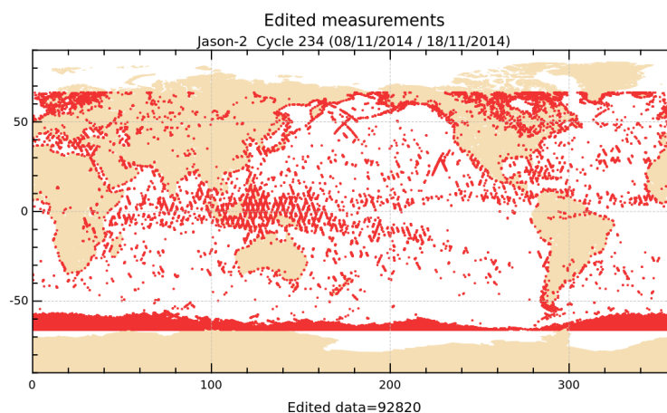
FIGURE 2 – Edited measurements for cycle 234.
