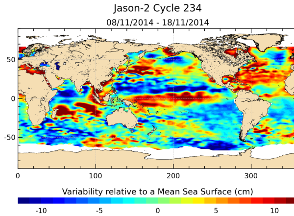
FIGURE 17 – Sea level anomaly relative to MSS for cycle 234.
