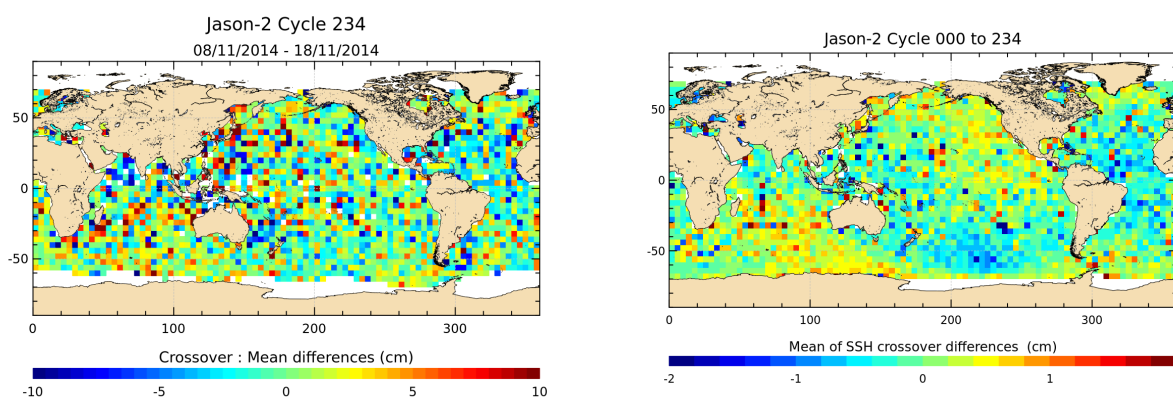
FIGURE 12 – Mean SSH at crossovers for cycle 234 (left) and over the whole Jason-2 period (right).
