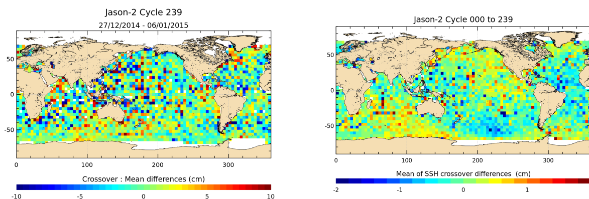
FIGURE 12 – Mean SSH at crossovers for cycle 239 (left) and over the whole Jason-2 period (right).
