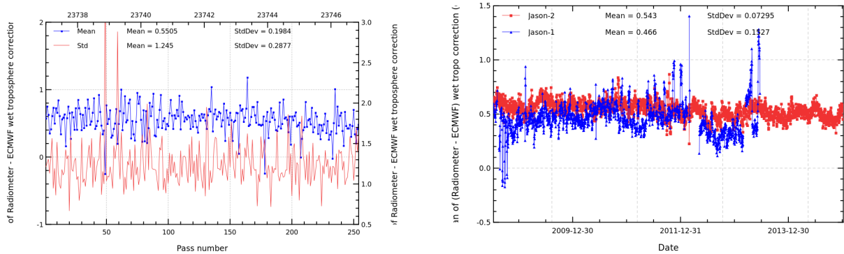
FIGURE 11 – Pass monitoring of wet troposphere differences between radiometer and ECMWF model for Jason-2 cycle 239 (left) and daily monitoring of wet troposphere differences between radiometer and ECMWF model (right).
