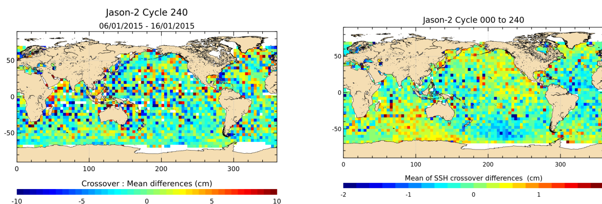
FIGURE 12 – Mean SSH at crossovers for cycle 240 (left) and over the whole Jason-2 period (right).
