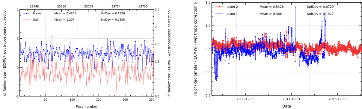
FIGURE 11 – Pass monitoring of wet troposphere differences between radiometer and ECMWF model for Jason-2 cycle 240 (left) and daily monitoring of wet troposphere differences between radiometer and ECMWF model (right).
