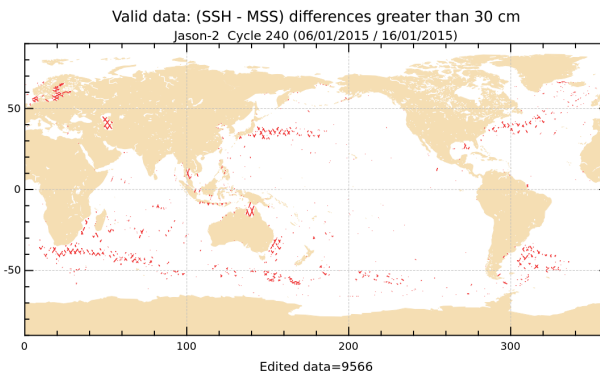
FIGURE 18 – Differences higher than a 30 cm threshold for cycle 240.
