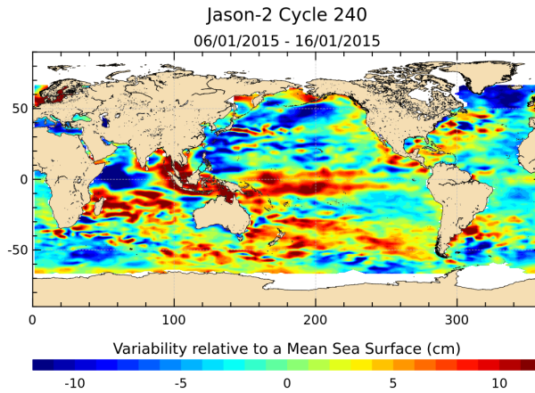
FIGURE 17 – Sea level anomaly relative to MSS for cycle 240.
