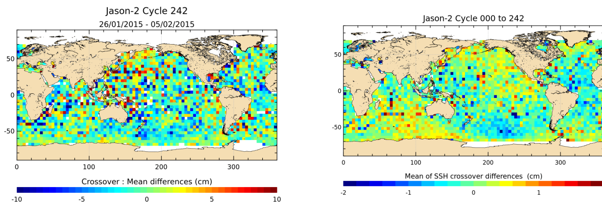
FIGURE 12 – Mean SSH at crossovers for cycle 242 (left) and over the whole Jason-2 period (right).
