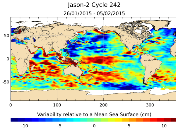
FIGURE 17 – Sea level anomaly relative to MSS for cycle 242.
