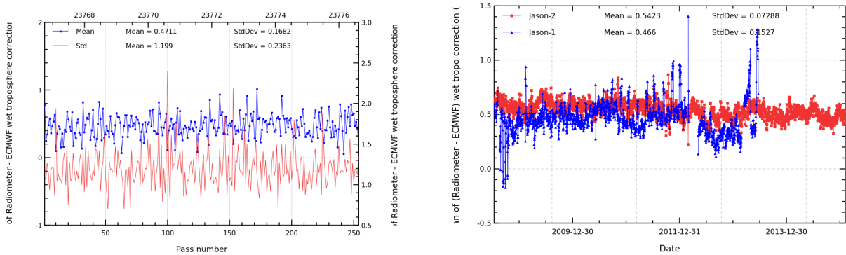
FIGURE 11 – Pass monitoring of wet troposphere differences between radiometer and ECMWF model for Jason-2 cycle 242 (left) and daily monitoring of wet troposphere differences between radiometer and ECMWF model (right).
