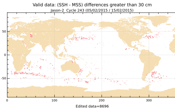
FIGURE 18 – Differences higher than a 30 cm threshold for cycle 243.
