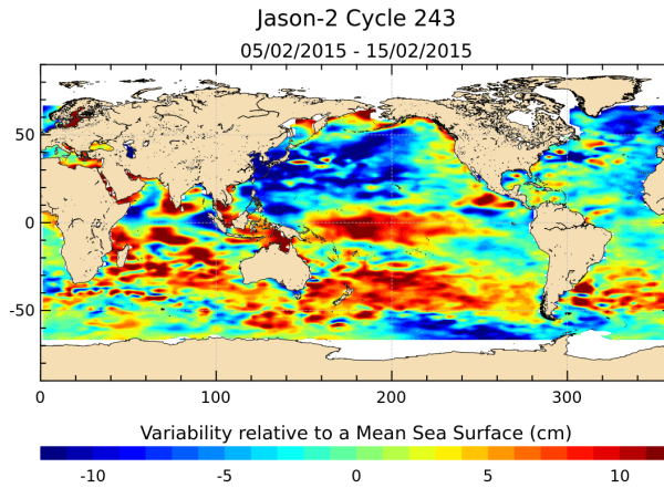
FIGURE 17 – Sea level anomaly relative to MSS for cycle 243.
