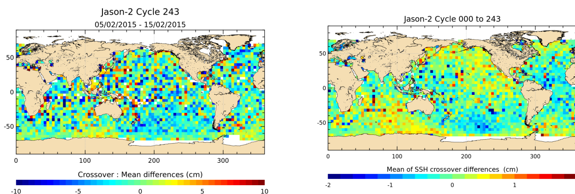
FIGURE 12 – Mean SSH at crossovers for cycle 243 (left) and over the whole Jason-2 period (right).
