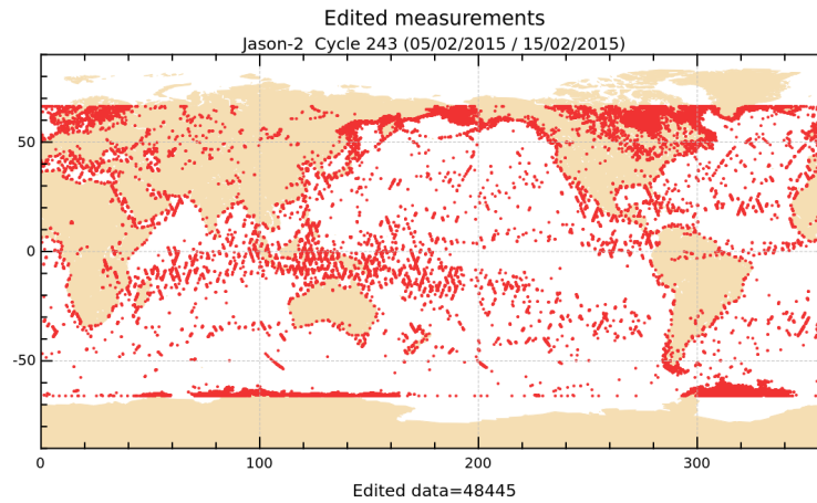
FIGURE 2 – Edited measurements for cycle 243.
