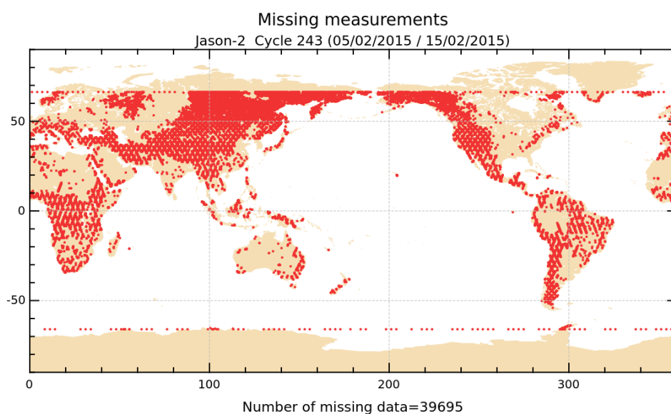
FIGURE 1 – Missing measurements for cycle 243.
