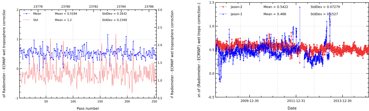
FIGURE 11 – Pass monitoring of wet troposphere differences between radiometer and ECMWF model for Jason-2 cycle 243 (left) and daily monitoring of wet troposphere differences between radiometer and ECMWF model (right).
