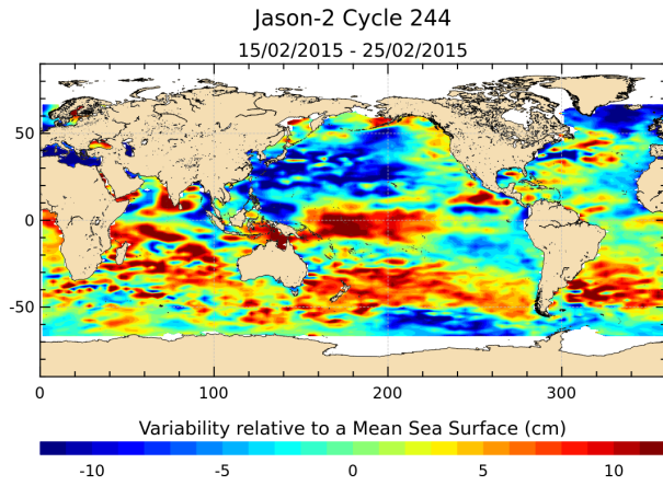
FIGURE 17 – Sea level anomaly relative to MSS for cycle 244.
