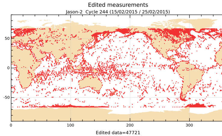
FIGURE 2 – Edited measurements for cycle 244.
