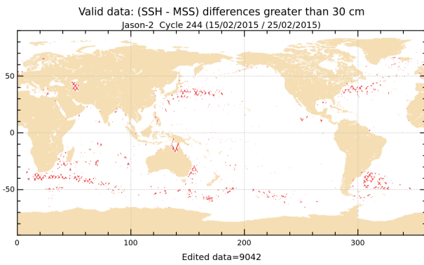
FIGURE 18 – Differences higher than a 30 cm threshold for cycle 244.
