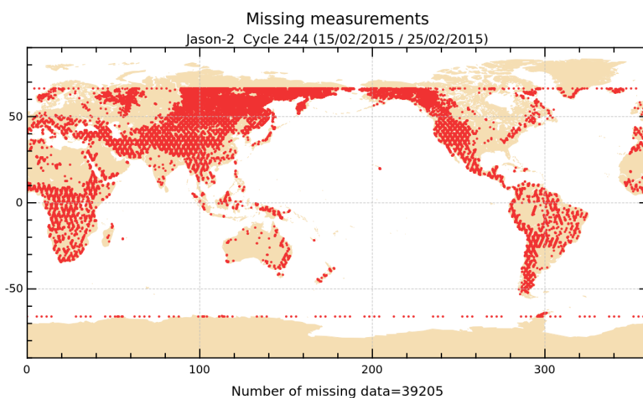
FIGURE 1 – Missing measurements for cycle 244.
