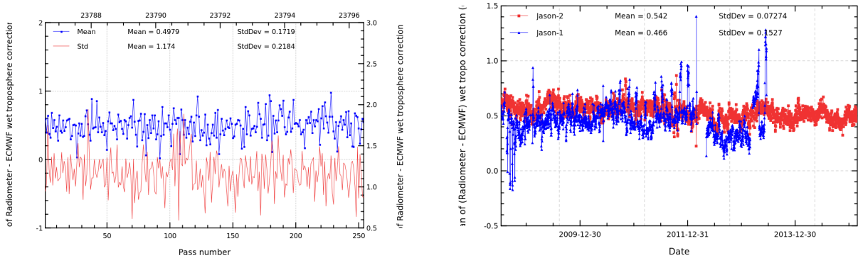
FIGURE 11 – Pass monitoring of wet troposphere differences between radiometer and ECMWF model for Jason-2 cycle 244 (left) and daily monitoring of wet troposphere differences between radiometer and ECMWF model (right).
