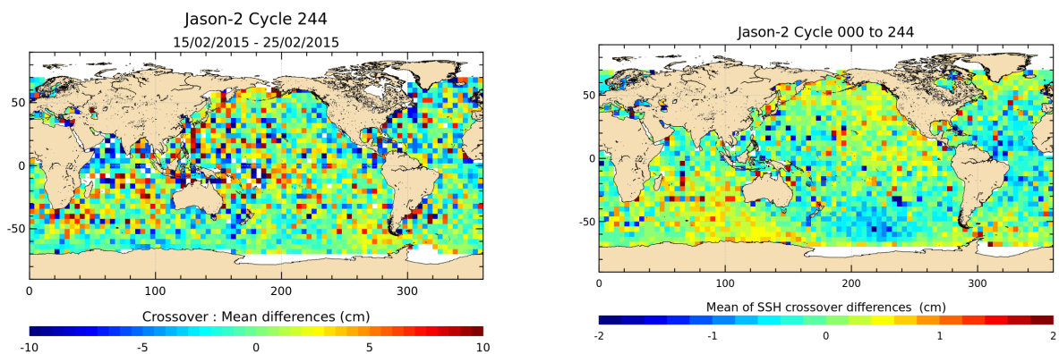
FIGURE 12 – Mean SSH at crossovers for cycle 244 (left) and over the whole Jason-2 period (right).
