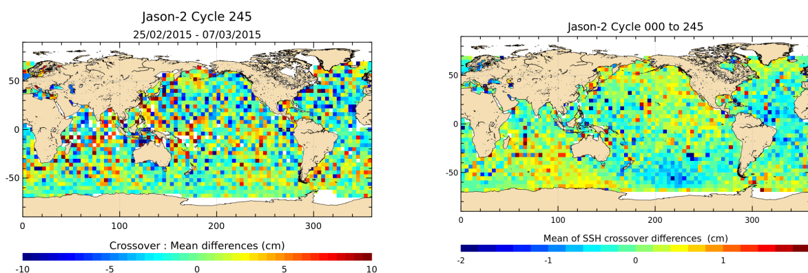
FIGURE 12 – Mean SSH at crossovers for cycle 245 (left) and over the whole Jason-2 period (right).
