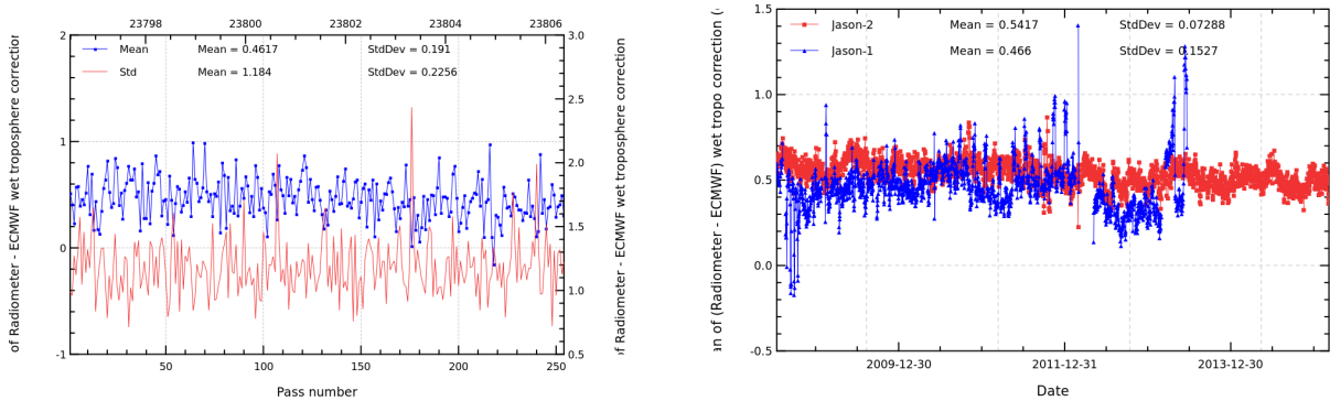
FIGURE 11 – Pass monitoring of wet troposphere differences between radiometer and ECMWF model for Jason-2 cycle 245 (left) and daily monitoring of wet troposphere differences between radiometer and ECMWF model (right).
