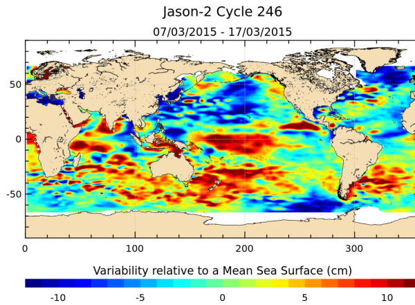
FIGURE 17 – Sea level anomaly relative to MSS for cycle 246.
