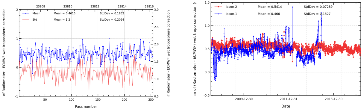
FIGURE 11 – Pass monitoring of wet troposphere differences between radiometer and ECMWF model for Jason-2 cycle 246 (left) and daily monitoring of wet troposphere differences between radiometer and ECMWF model (right).
