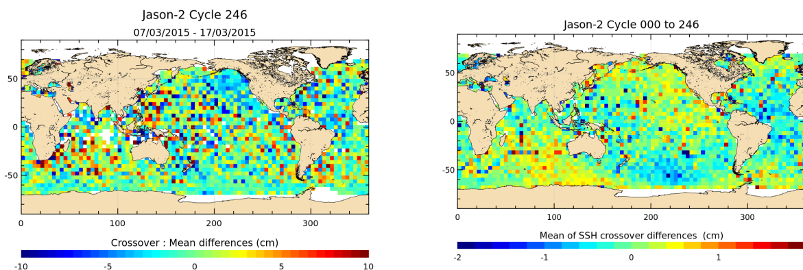
FIGURE 12 – Mean SSH at crossovers for cycle 246 (left) and over the whole Jason-2 period (right).
