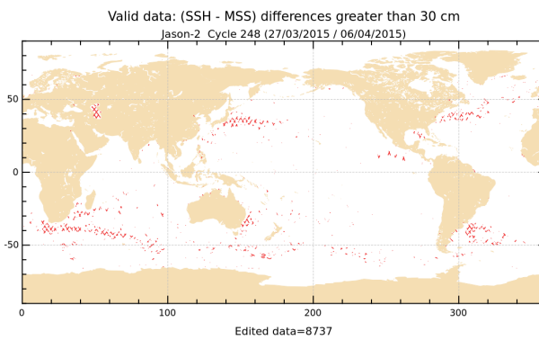
FIGURE 19 – Differences higher than a 30 cm threshold for cycle 248.
