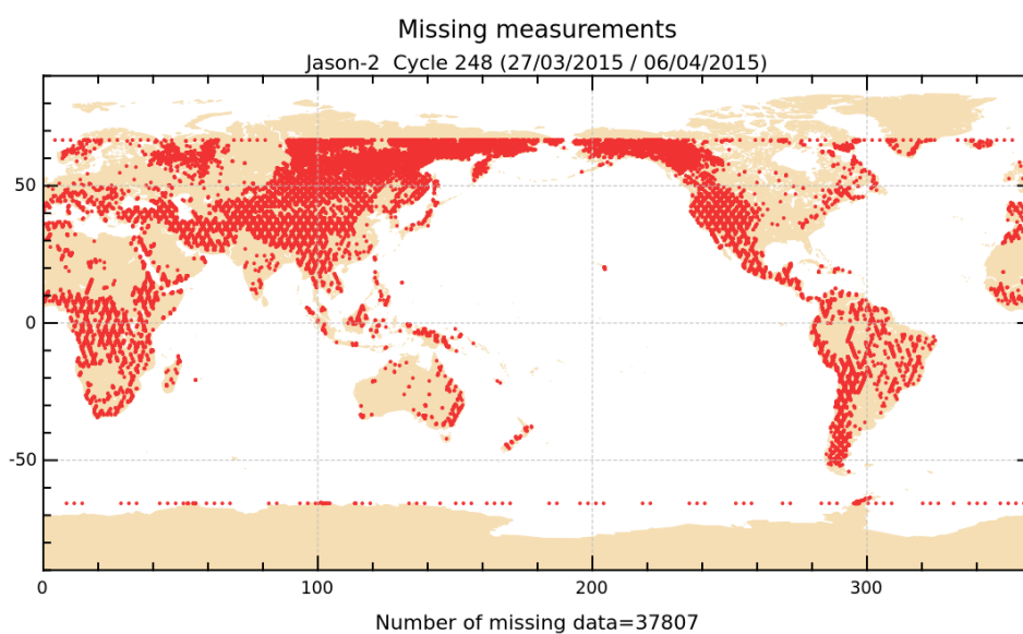
FIGURE 1 – Missing measurements for cycle 248.
