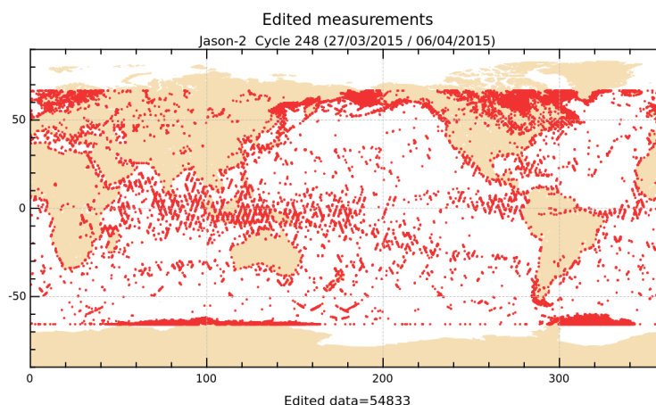
FIGURE 2 – Edited measurements for cycle 248.
