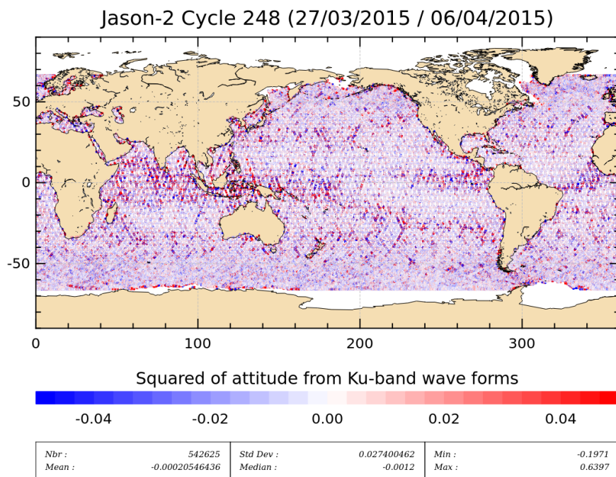
FIGURE 4 – Apparent squared mispointing from waveforms for cycle 248.
