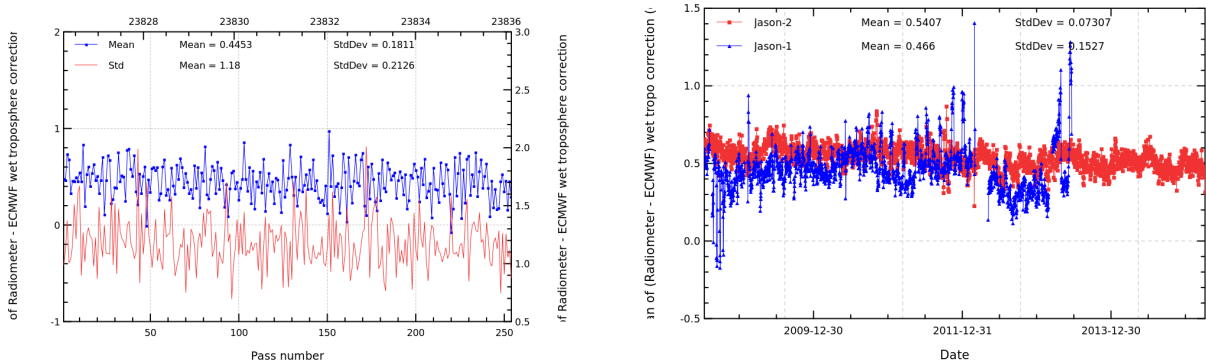
FIGURE 12 – Pass monitoring of wet troposphere differences between radiometer and ECMWF model for Jason-2 cycle 248 (left) and daily monitoring of wet troposphere differences between radiometer and ECMWF model (right).
