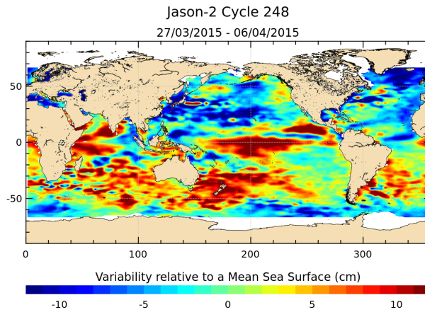
FIGURE 18 – Sea level anomaly relative to MSS for cycle 248.
