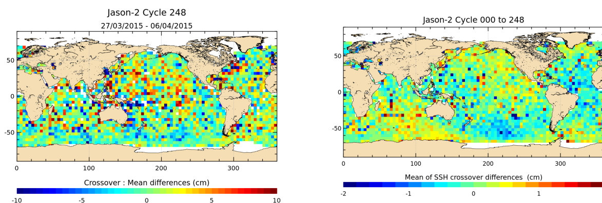
FIGURE 13 – Mean SSH at crossovers for cycle 248 (left) and over the whole Jason-2 period (right).
