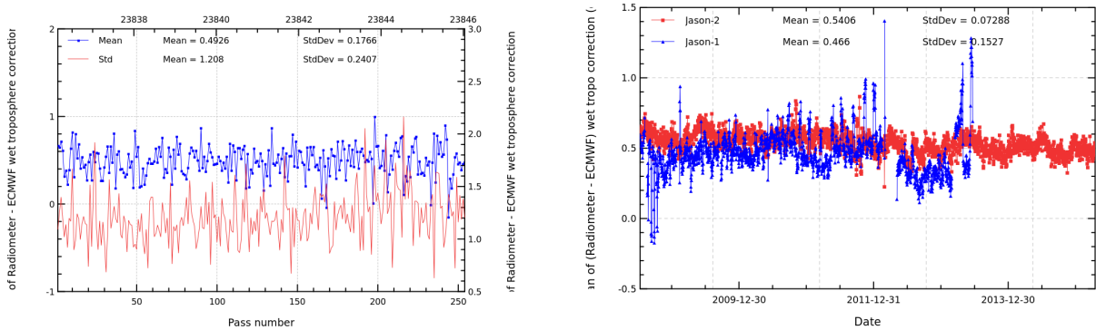
FIGURE 11 – Pass monitoring of wet troposphere differences between radiometer and ECMWF model for Jason-2 cycle 249 (left) and daily monitoring of wet troposphere differences between radiometer and ECMWF model (right).
