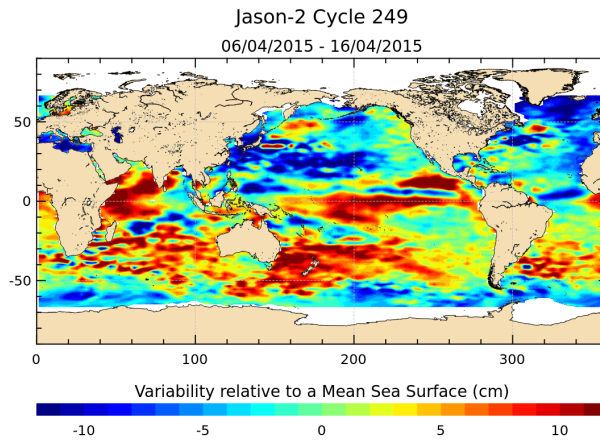
FIGURE 17 – Sea level anomaly relative to MSS for cycle 249.
