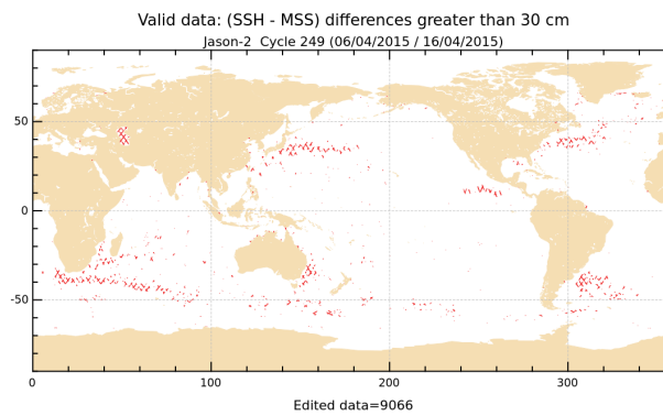
FIGURE 18 – Differences higher than a 30 cm threshold for cycle 249.
