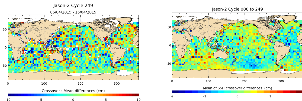
FIGURE 12 – Mean SSH at crossovers for cycle 249 (left) and over the whole Jason-2 period (right).
