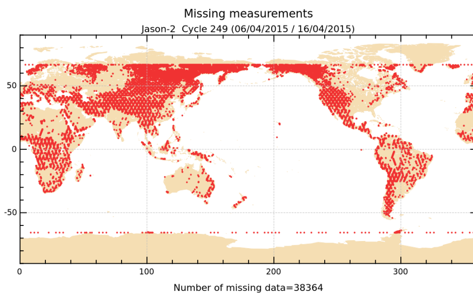
FIGURE 1 – Missing measurements for cycle 249.
