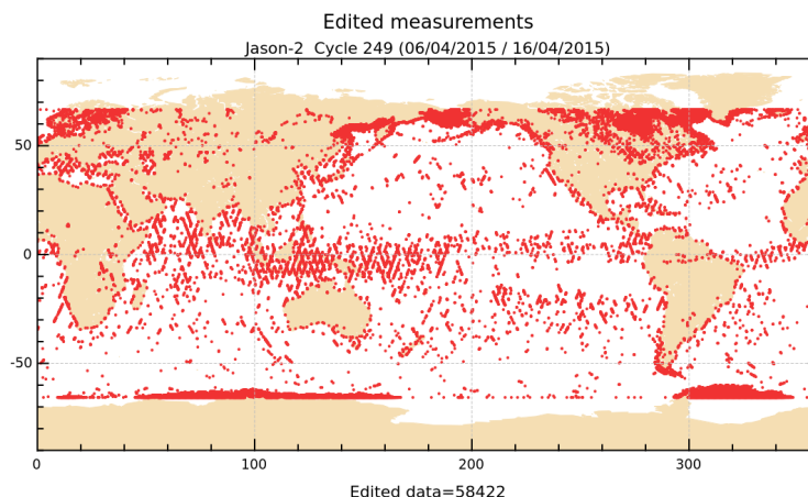
FIGURE 2 – Edited measurements for cycle 249.
