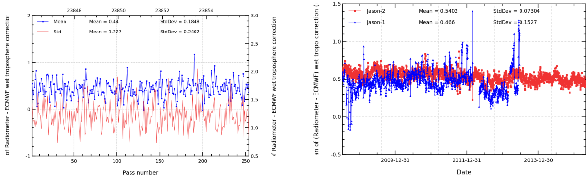
FIGURE 11 – Pass monitoring of wet troposphere differences between radiometer and ECMWF model for Jason-2 cycle 250 (left) and daily monitoring of wet troposphere differences between radiometer and ECMWF model (right).
