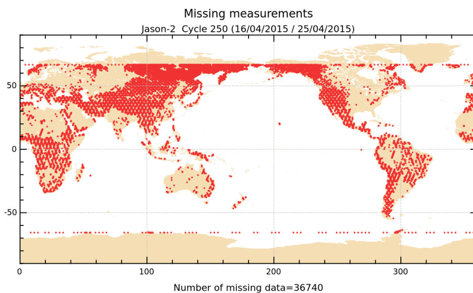
FIGURE 1 – Missing measurements for cycle 250.
