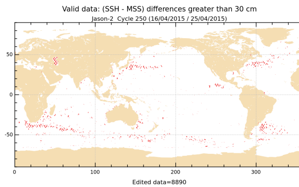
FIGURE 18 – Differences higher than a 30 cm threshold for cycle 250.
