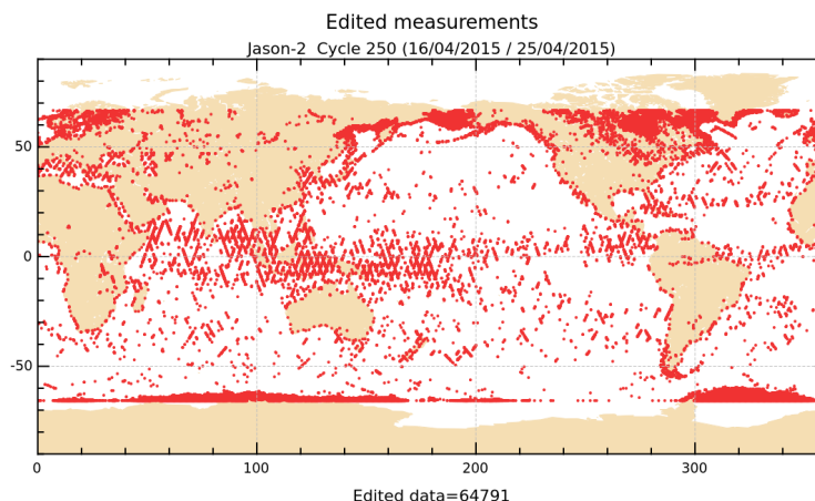
FIGURE 2 – Edited measurements for cycle 250.
