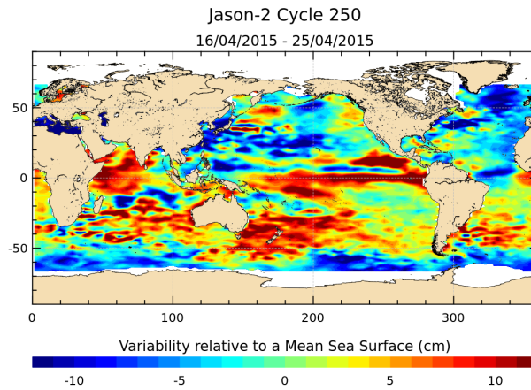
FIGURE 17 – Sea level anomaly relative to MSS for cycle 250.
