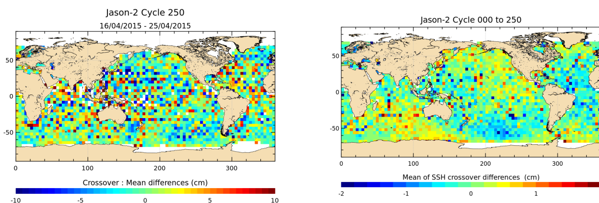
FIGURE 12 – Mean SSH at crossovers for cycle 250 (left) and over the whole Jason-2 period (right).
