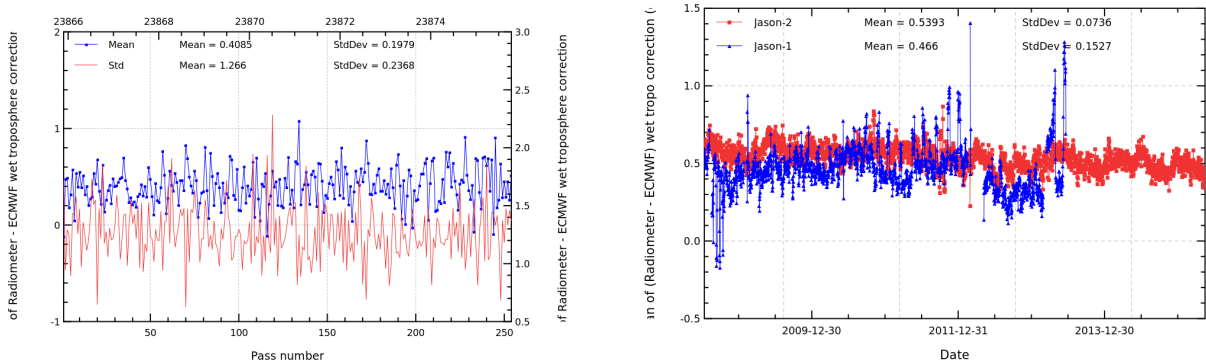
FIGURE 11 – Pass monitoring of wet troposphere differences between radiometer and ECMWF model for Jason-2 cycle 252 (left) and daily monitoring of wet troposphere differences between radiometer and ECMWF model (right).
