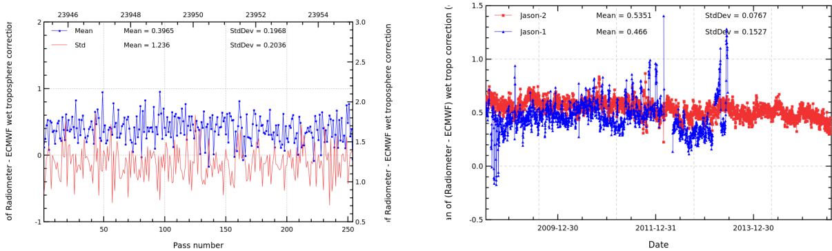
FIGURE 11 – Pass monitoring of wet troposphere differences between radiometer and ECMWF model for Jason-2 cycle 260 (left) and daily monitoring of wet troposphere differences between radiometer and ECMWF model (right).
