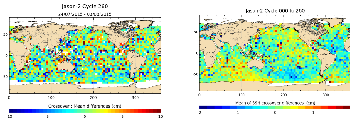
FIGURE 12 – Mean SSH at crossovers for cycle 260 (left) and over the whole Jason-2 period (right).
