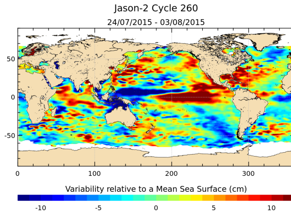
FIGURE 17 – Sea level anomaly relative to MSS for cycle 260.
