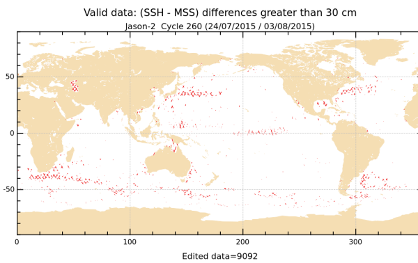
FIGURE 18 – Differences higher than a 30 cm threshold for cycle 260.
