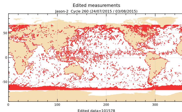
FIGURE 2 – Edited measurements for cycle 260.
