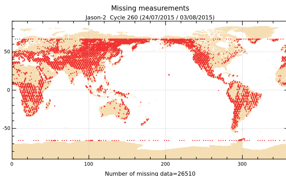
FIGURE 1 – Missing measurements for cycle 260.
