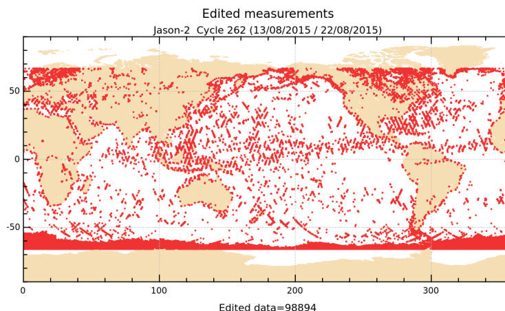
FIGURE 2 – Edited measurements for cycle 262.
