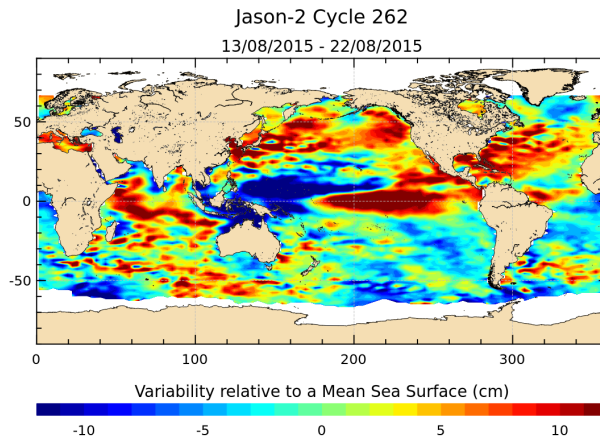
FIGURE 17 – Sea level anomaly relative to MSS for cycle 262.
