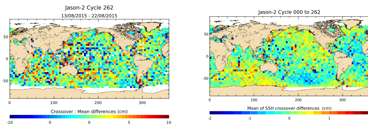
FIGURE 12 – Mean SSH at crossovers for cycle 262 (left) and over the whole Jason-2 period (right).
