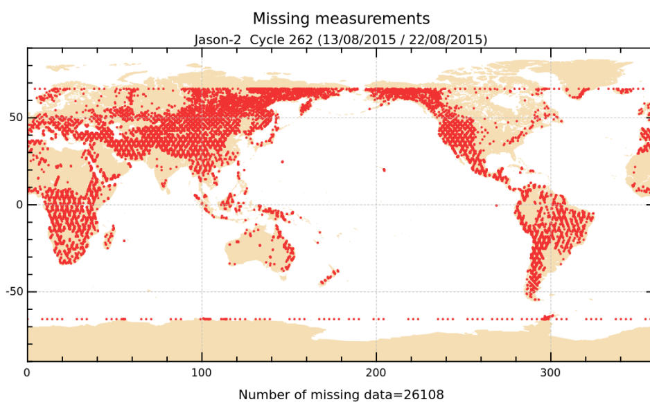
FIGURE 1 – Missing measurements for cycle 262.
