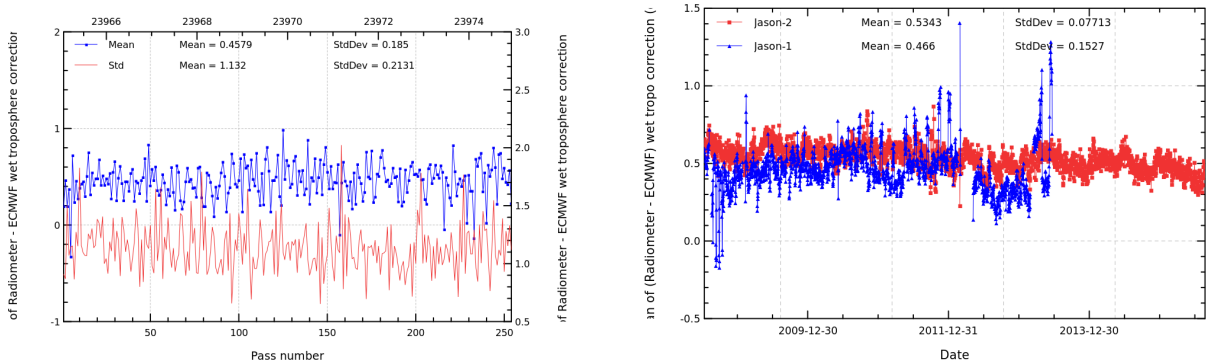
FIGURE 11 – Pass monitoring of wet troposphere differences between radiometer and ECMWF model for Jason-2 cycle 262 (left) and daily monitoring of wet troposphere differences between radiometer and ECMWF model (right).
