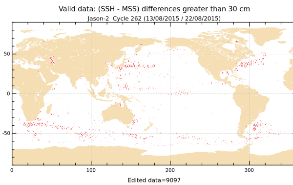
FIGURE 18 – Differences higher than a 30 cm threshold for cycle 262.
