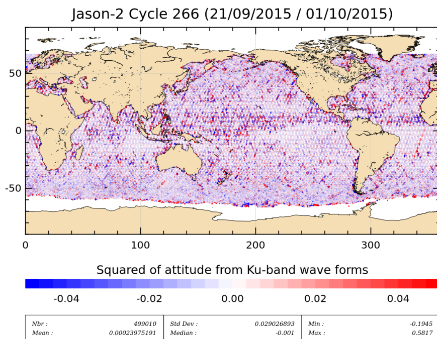
FIGURE 4 – Apparent squared mispointing from waveforms for cycle 266.
