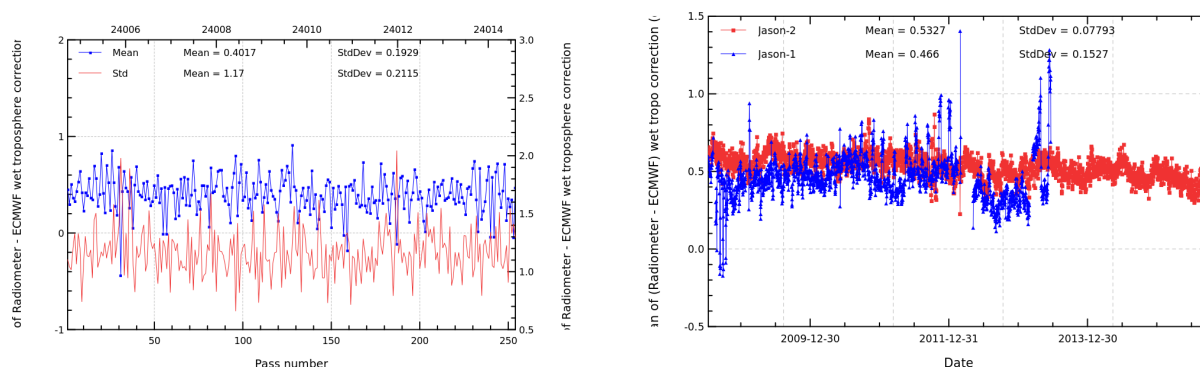
FIGURE 12 – Pass monitoring of wet troposphere differences between radiometer and ECMWF model for Jason-2 cycle 266 (left) and daily monitoring of wet troposphere differences between radiometer and ECMWF model (right).
