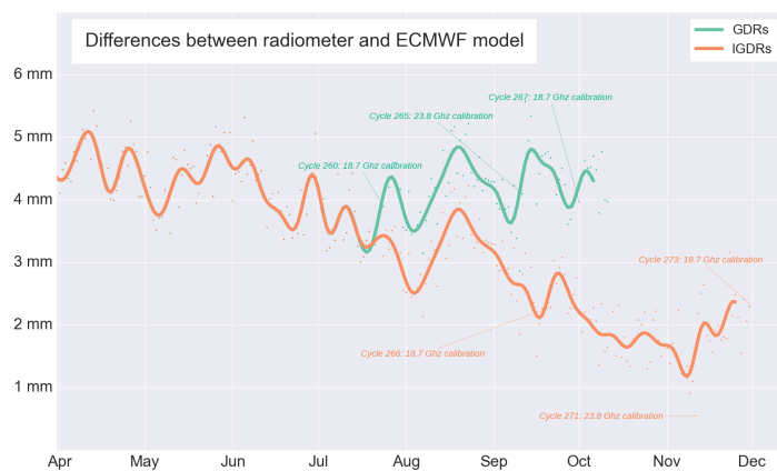
FIGURE 12 – Daily averaged difference between radiometer and ECMWF wet troposphere correction for Jason-2.
