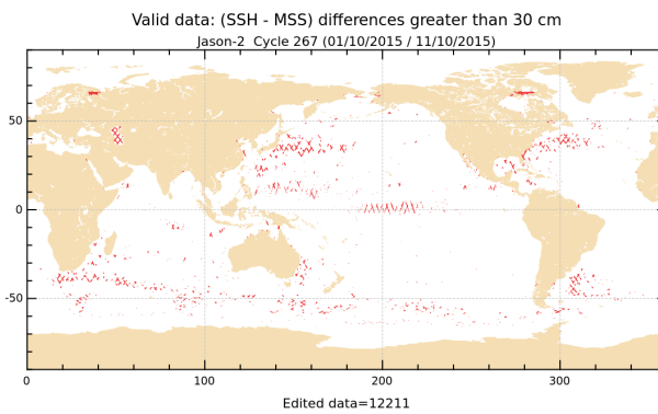
FIGURE 19 – Differences higher than a 30 cm threshold for cycle 267.
