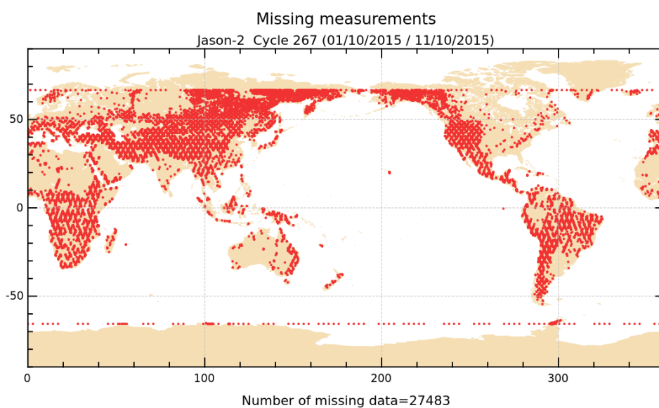
FIGURE 1 – Missing measurements for cycle 267.
