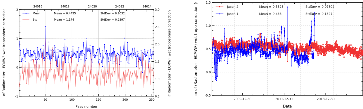
FIGURE 11 – Pass monitoring of wet troposphere differences between radiometer and ECMWF model for Jason-2 cycle 267 (left) and daily monitoring of wet troposphere differences between radiometer and ECMWF model (right).
