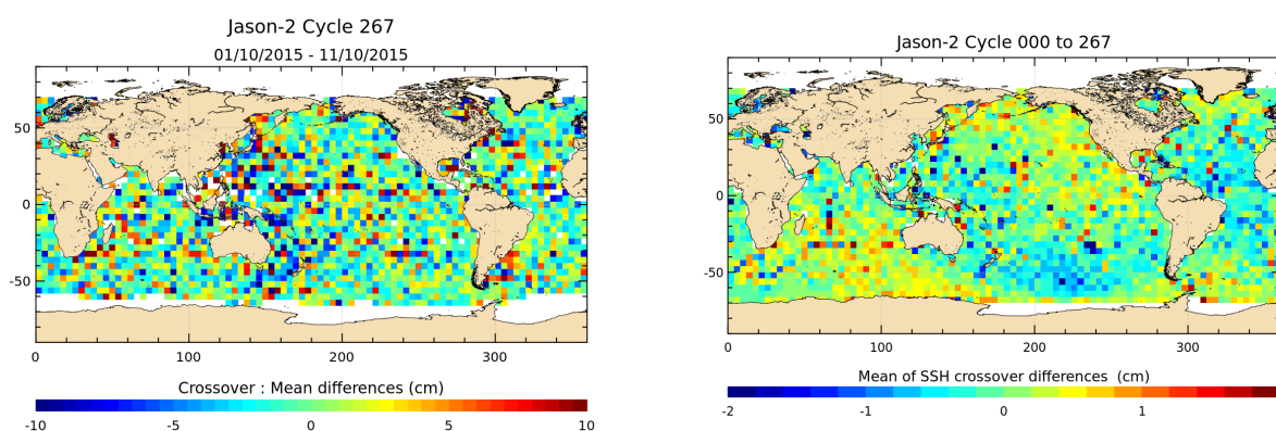
FIGURE 13 – Mean SSH at crossovers for cycle 267 (left) and over the whole Jason-2 period (right).
