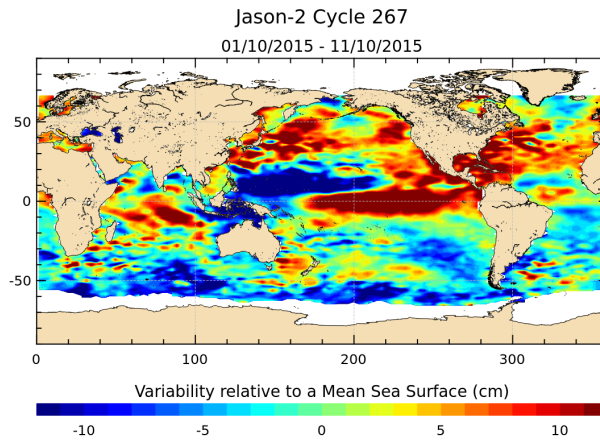
FIGURE 18 – Sea level anomaly relative to MSS for cycle 267.
