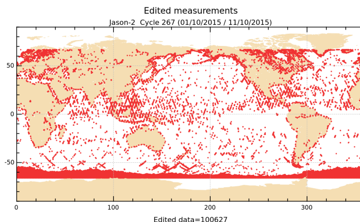
FIGURE 2 – Edited measurements for cycle 267.
