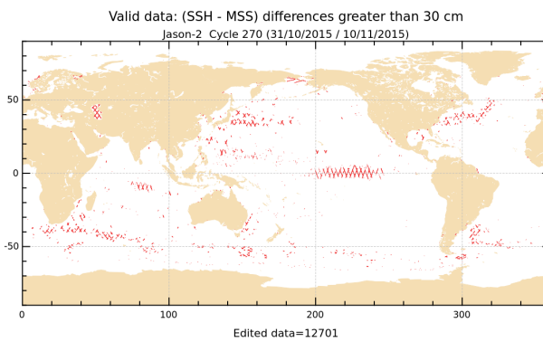
FIGURE 18 – Differences higher than a 30 cm threshold for cycle 270.
