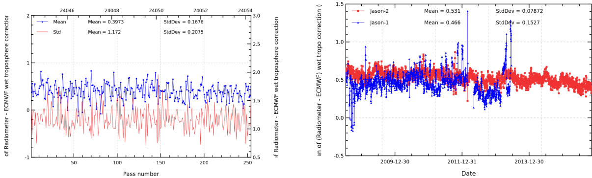
FIGURE 11 – Pass monitoring of wet troposphere differences between radiometer and ECMWF model for Jason-2 cycle 270 (left) and daily monitoring of wet troposphere differences between radiometer and ECMWF model (right).
