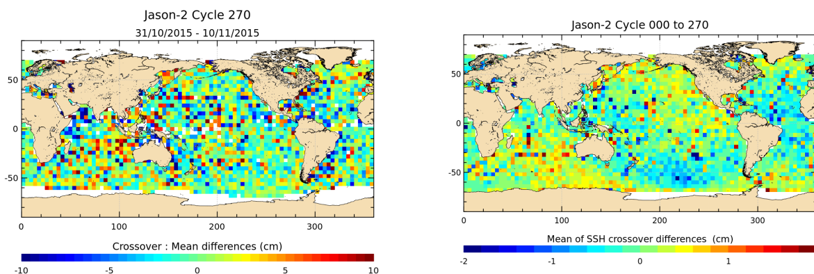
FIGURE 12 – Mean SSH at crossovers for cycle 270 (left) and over the whole Jason-2 period (right).
