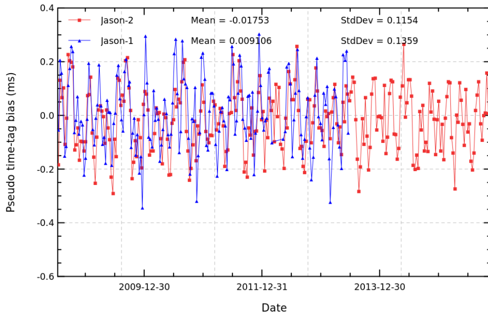
FIGURE 17 – Cyclic monitoring of pseudo time tag bias for Jason-1 and Jason-2.
