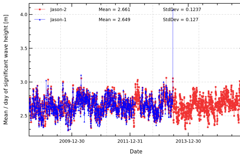
FIGURE 7 – Daily monitoring of Ku-band significant wave height for Jason-2 and Jason-1.
