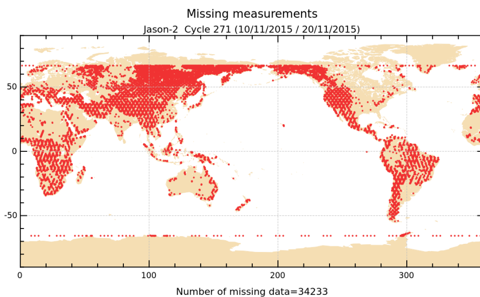
FIGURE 1 – Missing measurements for cycle 271.
