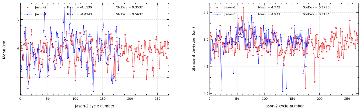
FIGURE 15 – Cyclic monitoring of mean (left) and standard deviation (right) of SSH differences at crossovers for Jason-1 and Jason-2.
