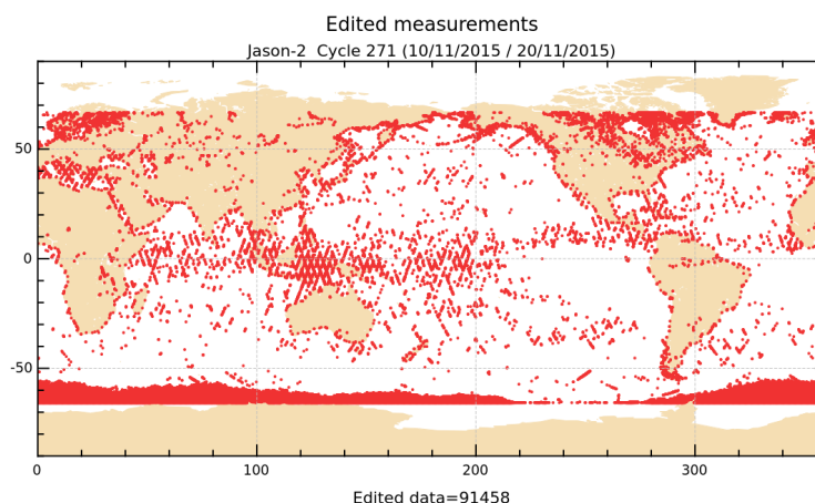
FIGURE 2 – Edited measurements for cycle 271.
