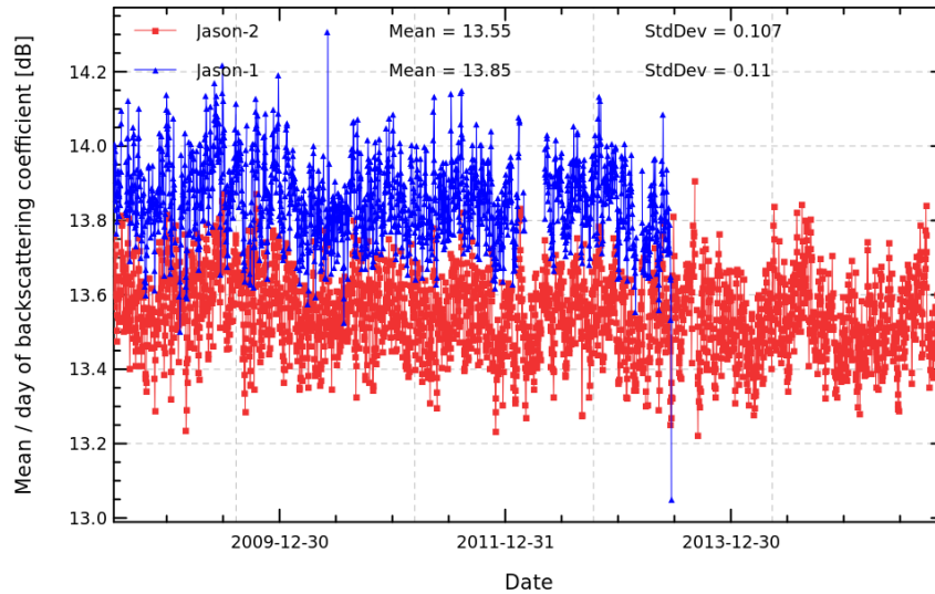
FIGURE 8 – Daily monitoring of Ku-band backscattering coefficient for Jason-2 and Jason-1.
