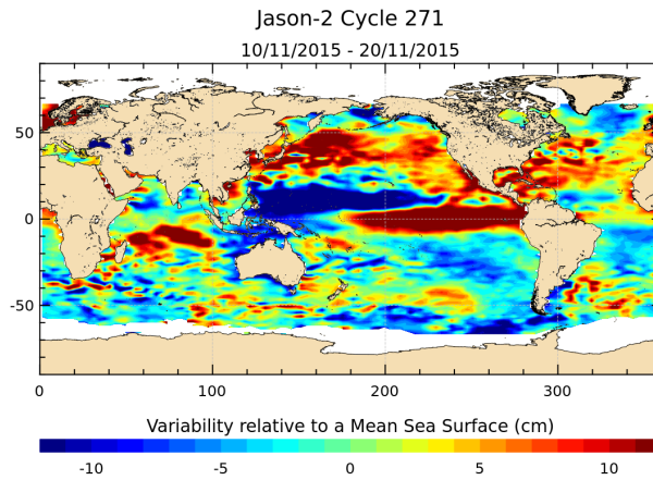
FIGURE 19 – Sea level anomaly relative to MSS for cycle 271.
