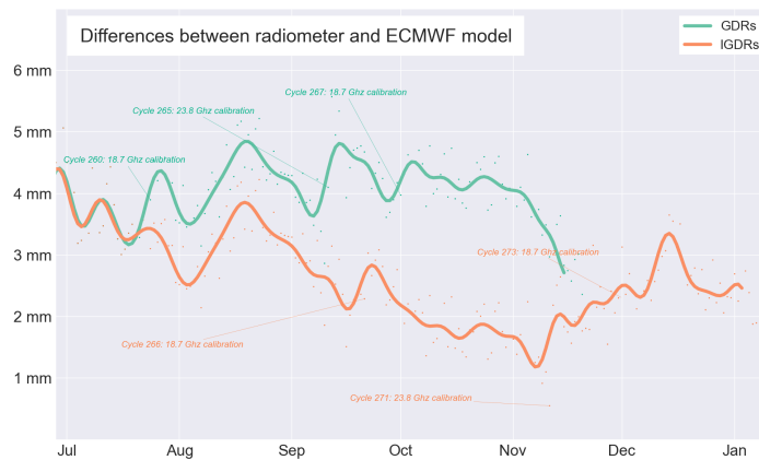
FIGURE 13 – Daily monitoring of wet tropospheric radiometer minus model corrections.
