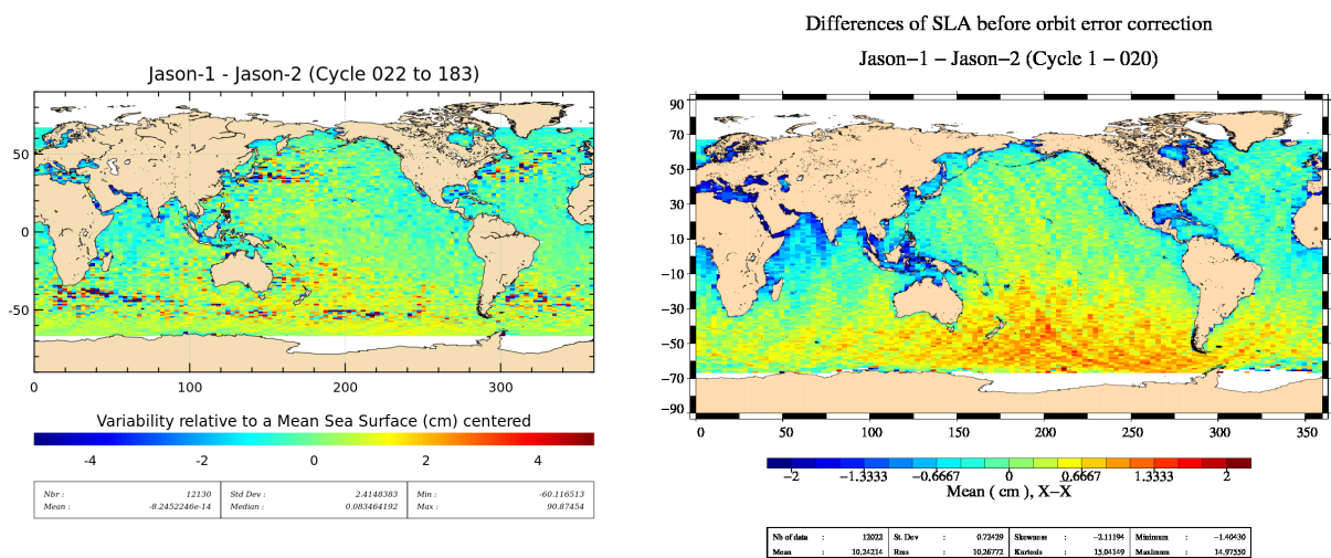
FIGURE 21 – Jason-1 – Jason-2 SLA differences averaged over whole Jason-2 period since cycle 022 until cycle 183 (left), and for flight formation phase (cycle 001 to 020) (right).
