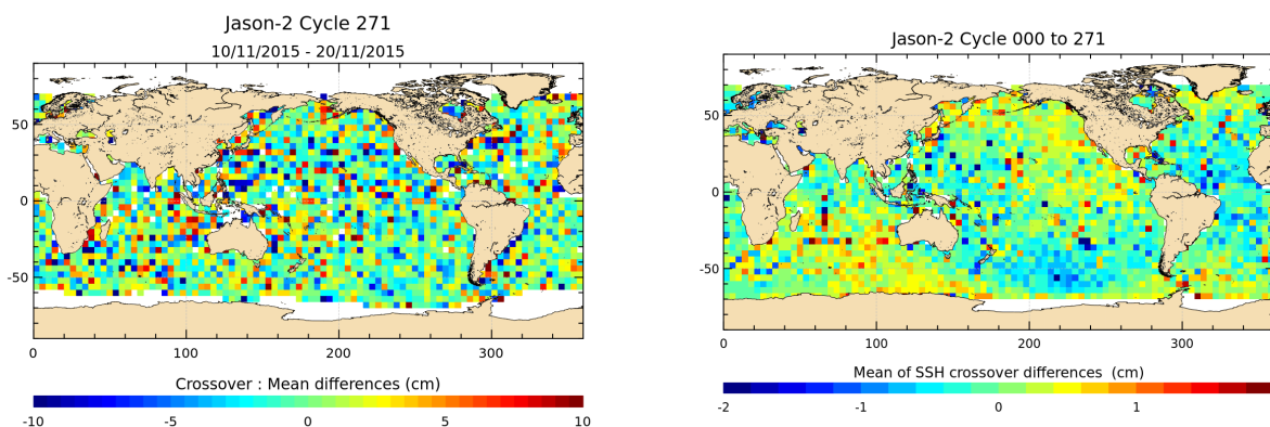
FIGURE 14 – Mean SSH at crossovers for cycle 271 (left) and over the whole Jason-2 period (right).
