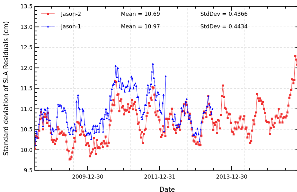
FIGURE 22 – Cyclic monitoring standard deviation of along track SLA for Jason-1 and Jason-2.
