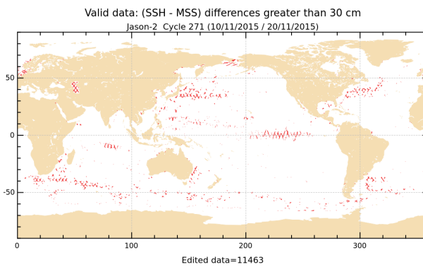
FIGURE 20 – Differences higher than a 30 cm threshold for cycle 271.
