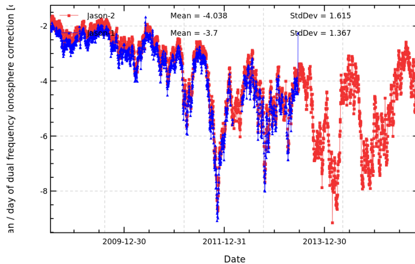
FIGURE 9 – Daily monitoring of dual-frequency ionosphere correction for Jason-2 and Jason-1.
