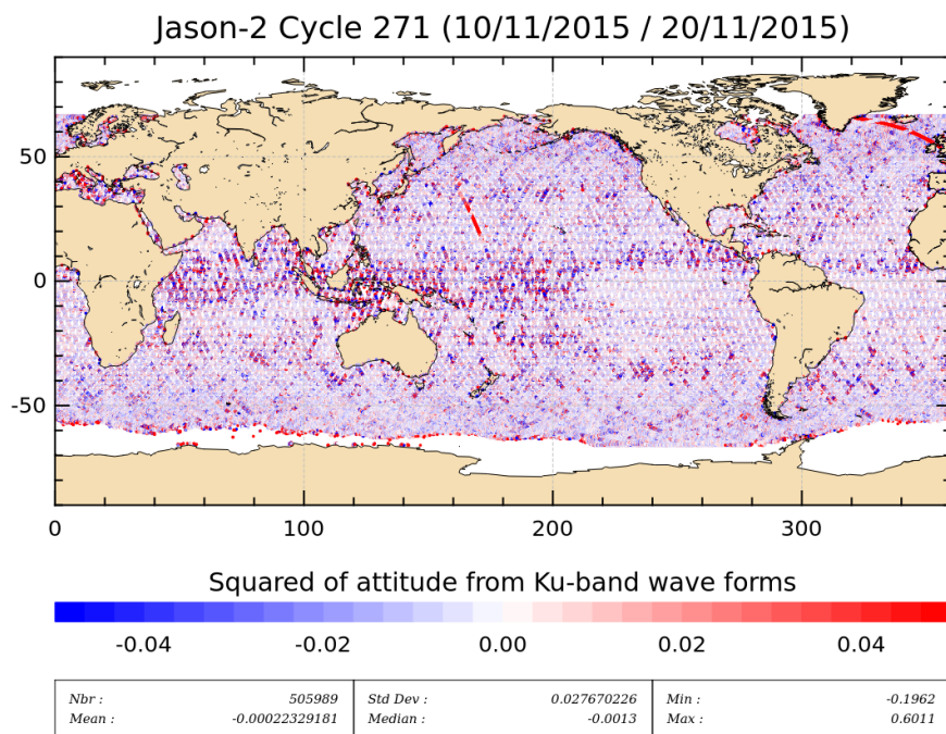
FIGURE 4 – Apparent squared mispointing from waveforms for cycle 271.
