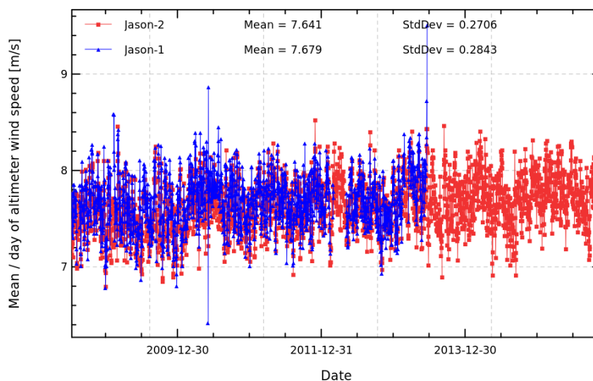
FIGURE 11 – Daily monitoring of altimeter wind speed for Jason-2 and Jason-1.
