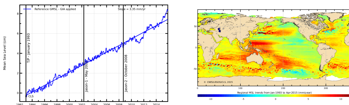
FIGURE 23 – Global (left) and regional (right) MSL trends from 1993 onwards.
