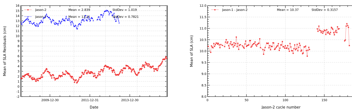
FIGURE 18 – Cyclic monitoring of mean SLA for Jason-1 and Jason-2 (left) and differences of (Jason-1 – Jason-2) mean SLA (right).
