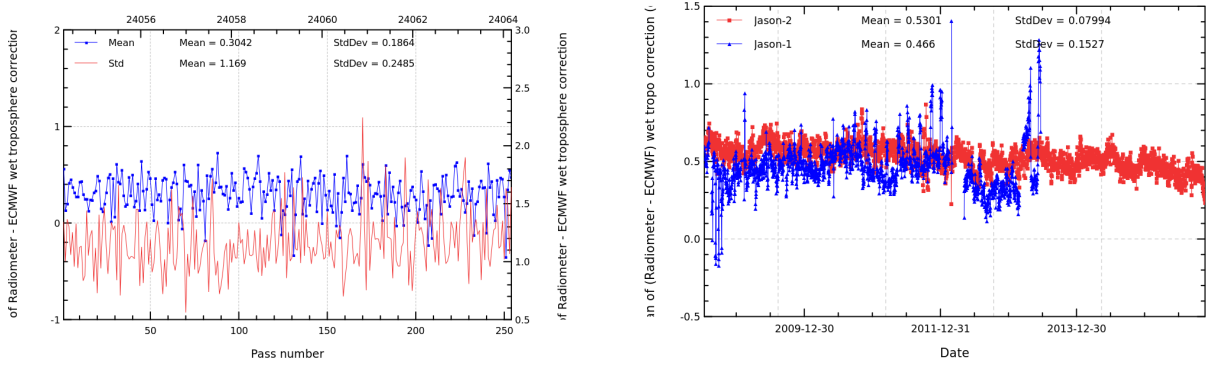
FIGURE 12 – Pass monitoring of wet troposphere differences between radiometer and ECMWF model for Jason-2 cycle 271 (left) and daily monitoring of wet troposphere differences between radiometer and ECMWF model (right).
