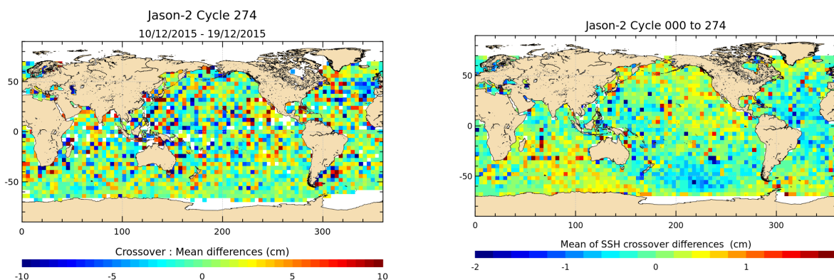
FIGURE 12 – Mean SSH at crossovers for cycle 274 (left) and over the whole Jason-2 period (right).
