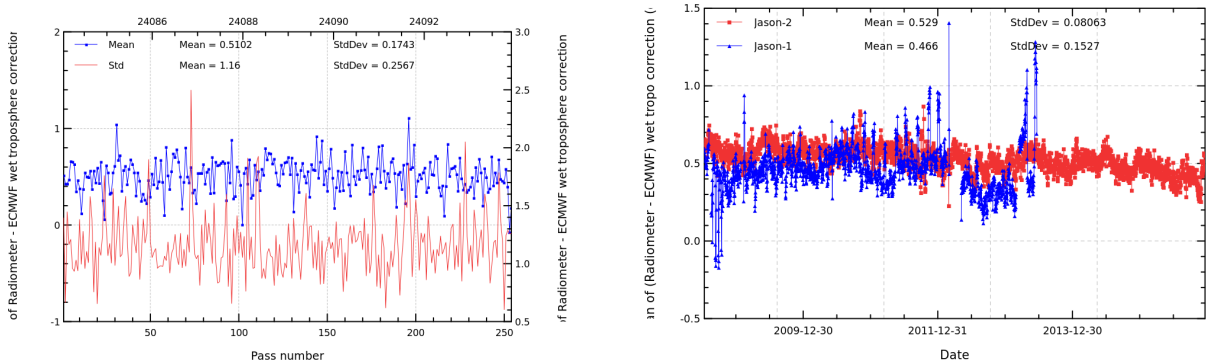
FIGURE 11 – Pass monitoring of wet troposphere differences between radiometer and ECMWF model for Jason-2 cycle 274 (left) and daily monitoring of wet troposphere differences between radiometer and ECMWF model (right).
