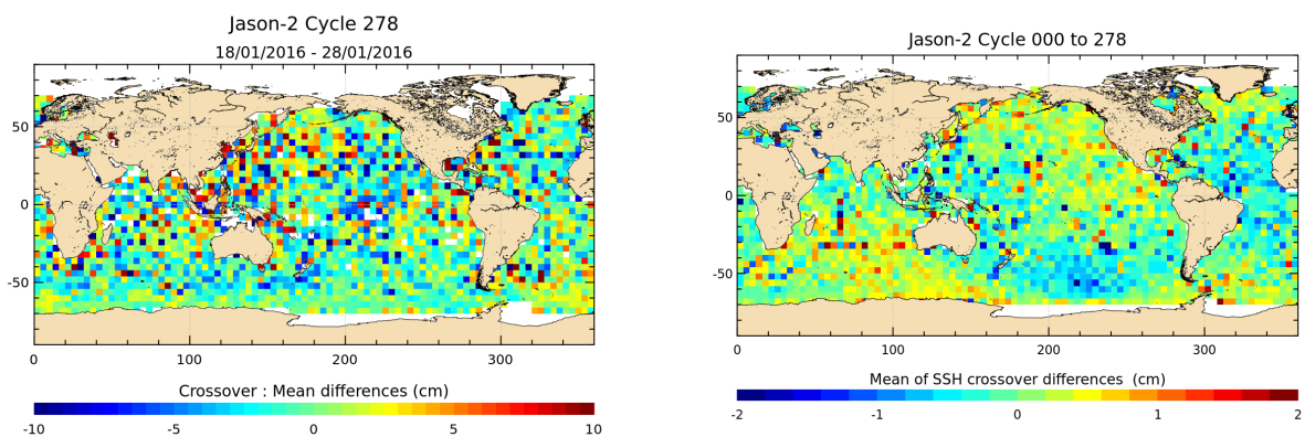
FIGURE 13 – Mean SSH at crossovers for cycle 278 (left) and over the whole Jason-2 period (right).
