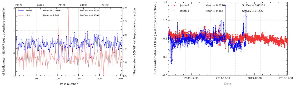
FIGURE 12 – Pass monitoring of wet troposphere differences between radiometer and ECMWF model for Jason-2 cycle 278 (left) and daily monitoring of wet troposphere differences between radiometer and ECMWF model (right).
