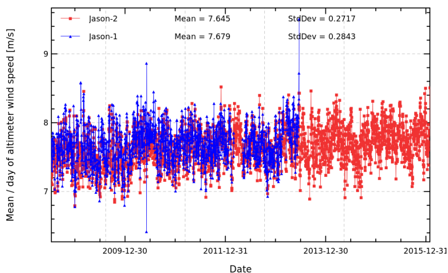
FIGURE 11 – Daily monitoring of altimeter wind speed for Jason-2 and Jason-1.
