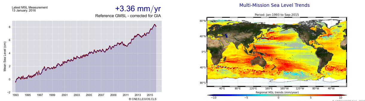
FIGURE 22 – Global (left) and regional (right) MSL trends from 1993 onwards.
