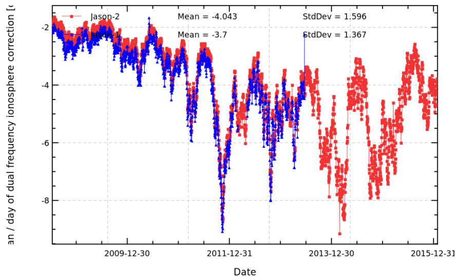
FIGURE 9 – Daily monitoring of dual-frequency ionosphere correction for Jason-2 and Jason-1.
