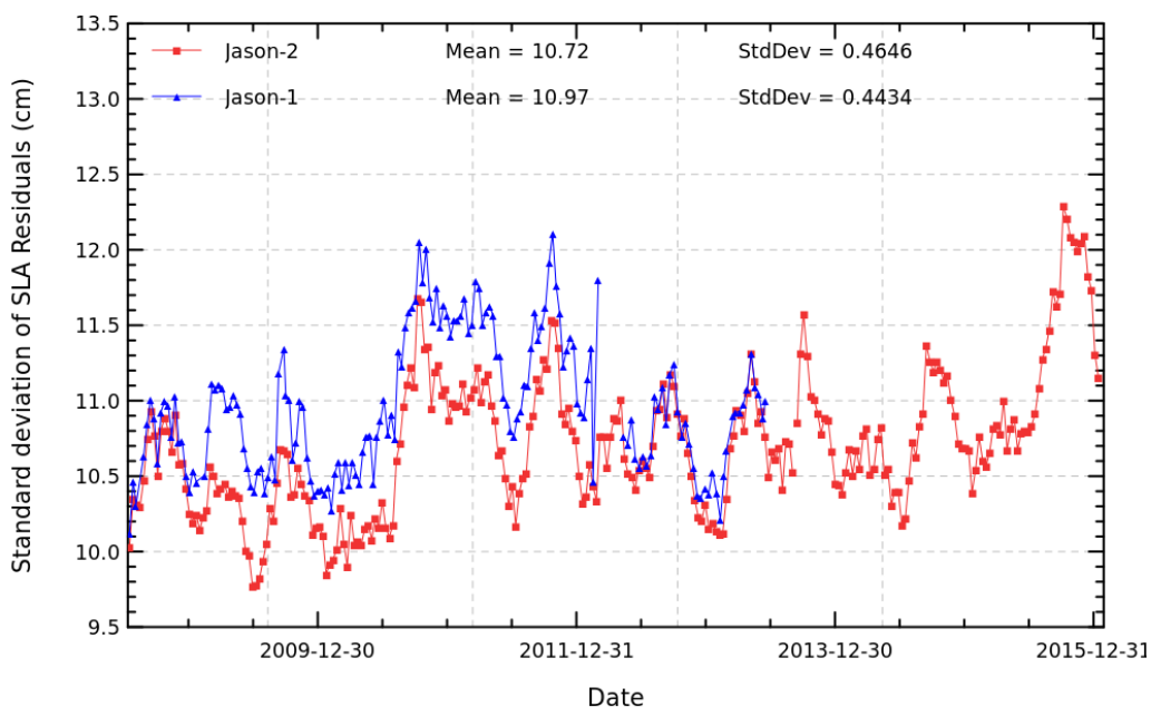
FIGURE 21 – Cyclic monitoring standard deviation of along track SLA for Jason-1 and Jason-2.
