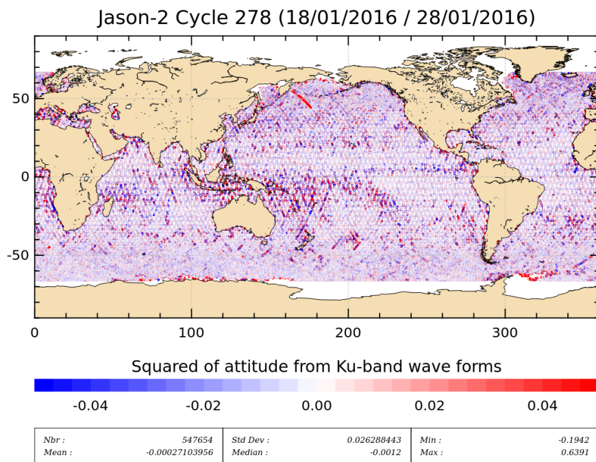
FIGURE 4 – Apparent squared mispointing from waveforms for cycle 278.
