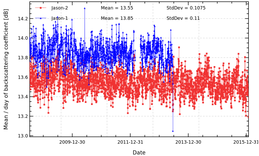
FIGURE 8 – Daily monitoring of Ku-band backscattering coefficient for Jason-2 and Jason-1.
