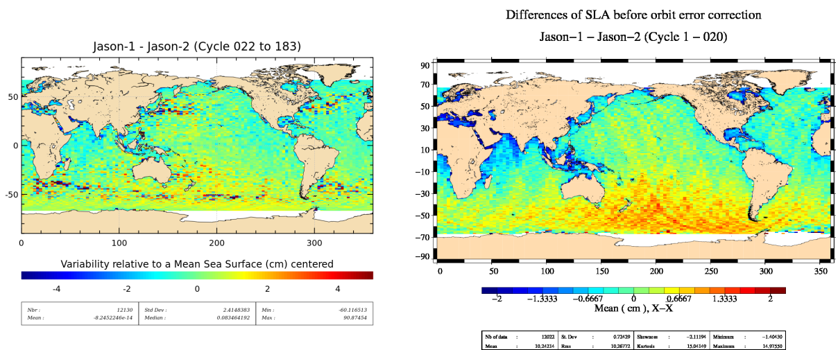
FIGURE 20 – Jason-1 – Jason-2 SLA differences averaged over whole Jason-2 period since cycle 022 until cycle 183 (left), and for flight formation phase (cycle 001 to 020) (right).
