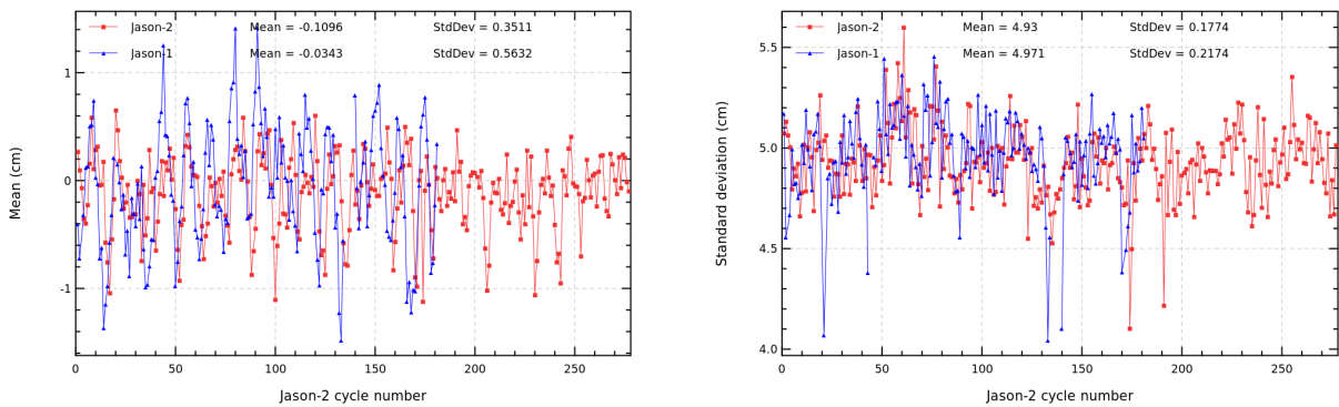
FIGURE 14 – Cyclic monitoring of mean (left) and standard deviation (right) of SSH differences at crossovers for Jason-1 and Jason-2.
