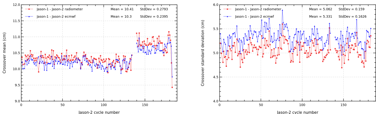
FIGURE 15 – Cyclic monitoring of mean (left) and standard deviation (right) of (Jason-1 – Jason-2) SSH differences at crossovers.
