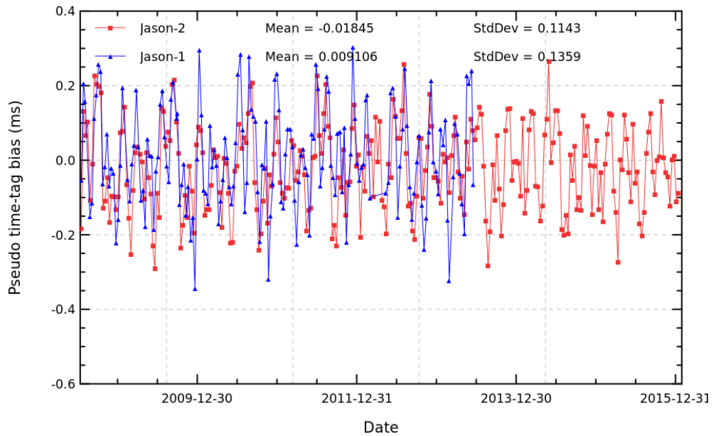
FIGURE 16 – Cyclic monitoring of pseudo time tag bias for Jason-1 and Jason-2.
