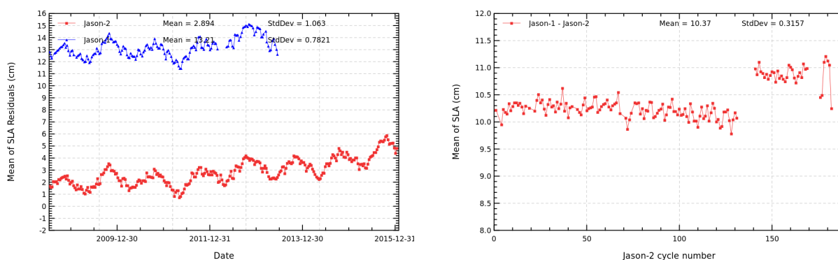
FIGURE 17 – Cyclic monitoring of mean SLA for Jason-1 and Jason-2 (left) and differences of (Jason-1 – Jason-2) mean SLA (right).
