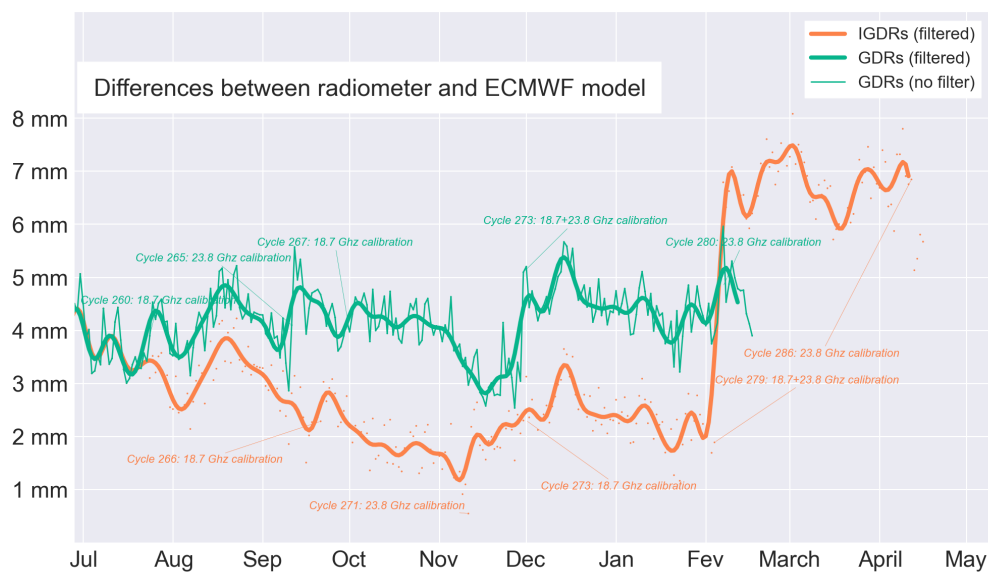
FIGURE 12 – Daily monitoring of radiometer minus ECMWF model wet troposphere difference.
