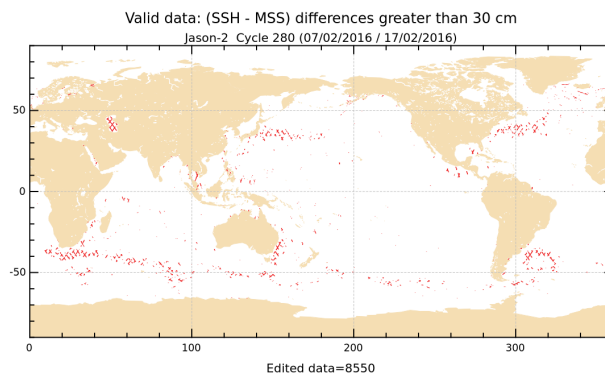
FIGURE 19 – Differences higher than a 30 cm threshold for cycle 280.
