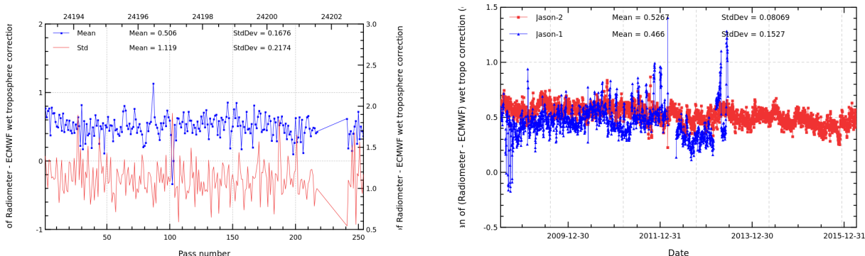
FIGURE 11 – Pass monitoring of wet troposphere differences between radiometer and ECMWF model for Jason-2 cycle 285 (left) and daily monitoring of wet troposphere differences between radiometer and ECMWF model (right).
