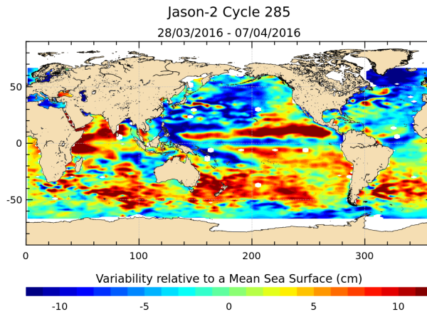
FIGURE 17 – Sea level anomaly relative to MSS for cycle 285.
