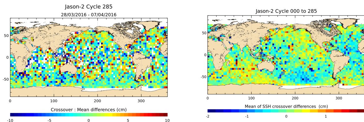
FIGURE 12 – Mean SSH at crossovers for cycle 285 (left) and over the whole Jason-2 period (right).
