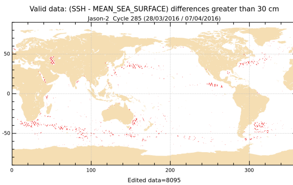
FIGURE 18 – Differences higher than a 30 cm threshold for cycle 285.
