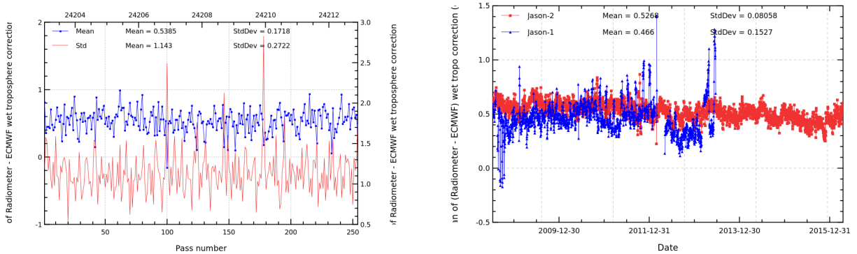
FIGURE 11 – Pass monitoring of wet troposphere differences between radiometer and ECMWF model for Jason-2 cycle 286 (left) and daily monitoring of wet troposphere differences between radiometer and ECMWF model (right).
