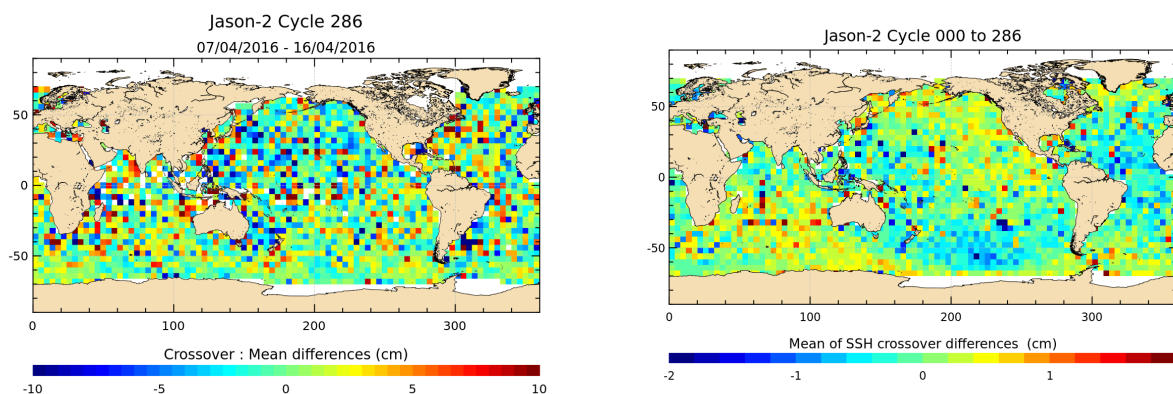
FIGURE 12 – Mean SSH at crossovers for cycle 286 (left) and over the whole Jason-2 period (right).
