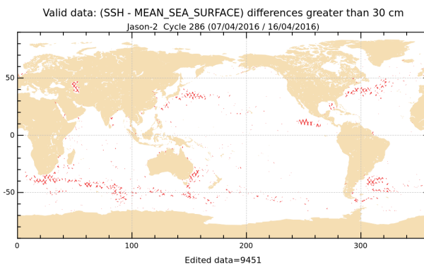
FIGURE 18 – Differences higher than a 30 cm threshold for cycle 286.
