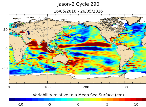
FIGURE 17 – Sea level anomaly relative to MSS for cycle 290.
