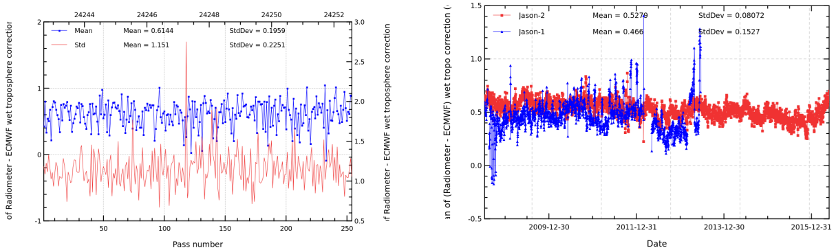
FIGURE 11 – Pass monitoring of wet troposphere differences between radiometer and ECMWF model for Jason-2 cycle 290 (left) and daily monitoring of wet troposphere differences between radiometer and ECMWF model (right).
