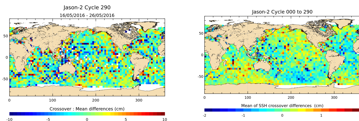
FIGURE 12 – Mean SSH at crossovers for cycle 290 (left) and over the whole Jason-2 period (right).
