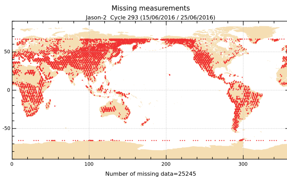
FIGURE 1 – Missing measurements for cycle 293.
