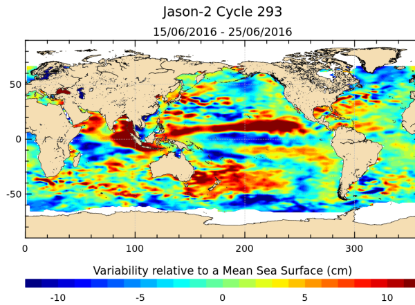
FIGURE 17 – Sea level anomaly relative to MSS for cycle 293.
