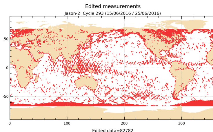
FIGURE 2 – Edited measurements for cycle 293.
