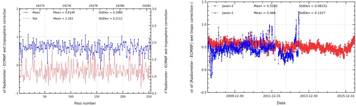
FIGURE 11 – Pass monitoring of wet troposphere differences between radiometer and ECMWF model for Jason-2 cycle 293 (left) and daily monitoring of wet troposphere differences between radiometer and ECMWF model (right).
