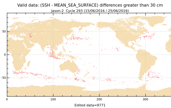
FIGURE 18 – Differences higher than a 30 cm threshold for cycle 293.
