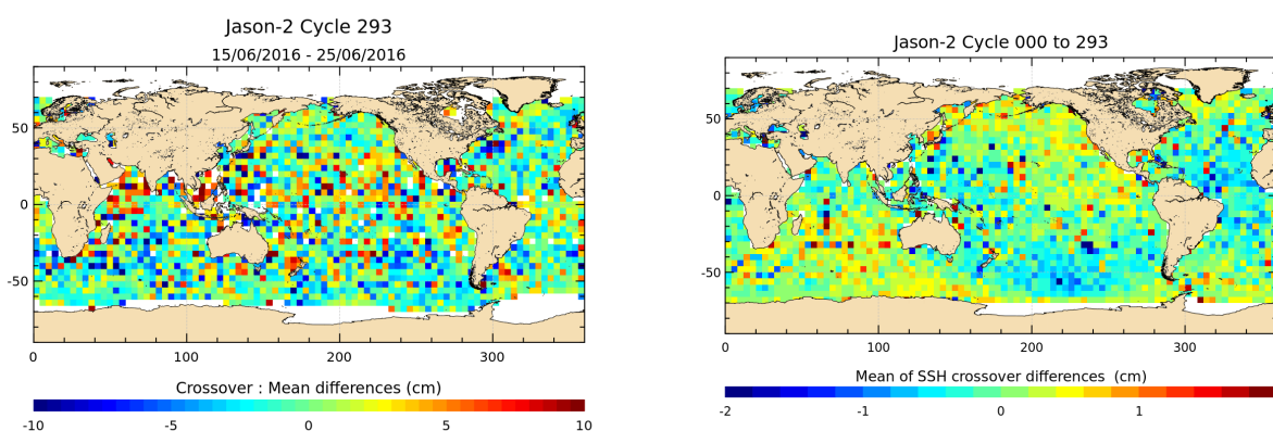
FIGURE 12 – Mean SSH at crossovers for cycle 293 (left) and over the whole Jason-2 period (right).
