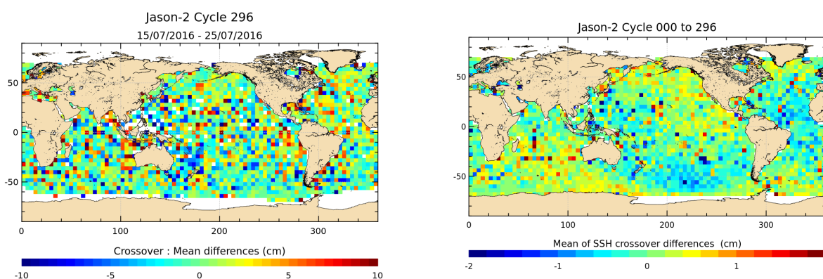
FIGURE 12 – Mean SSH at crossovers for cycle 296 (left) and over the whole Jason-2 period (right).
