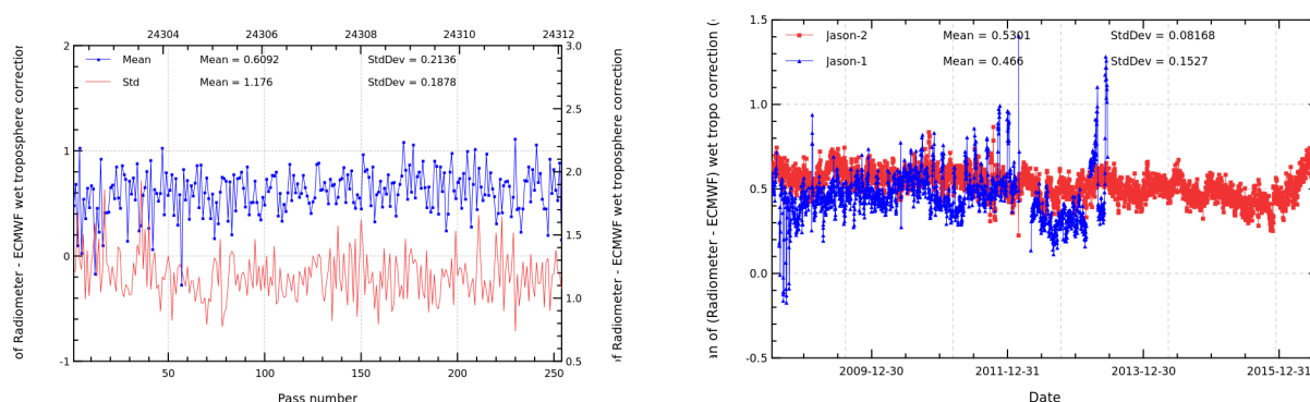
FIGURE 11 – Pass monitoring of wet troposphere differences between radiometer and ECMWF model for Jason-2 cycle 296 (left) and daily monitoring of wet troposphere differences between radiometer and ECMWF model (right).
