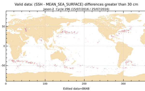
FIGURE 18 – Differences higher than a 30 cm threshold for cycle 296.
