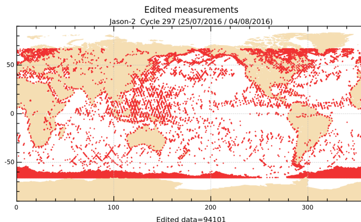
FIGURE 2 – Edited measurements for cycle 297.
