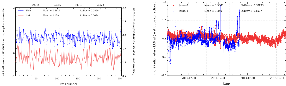
FIGURE 11 – Pass monitoring of wet troposphere differences between radiometer and ECMWF model for Jason-2 cycle 297 (left) and daily monitoring of wet troposphere differences between radiometer and ECMWF model (right).
