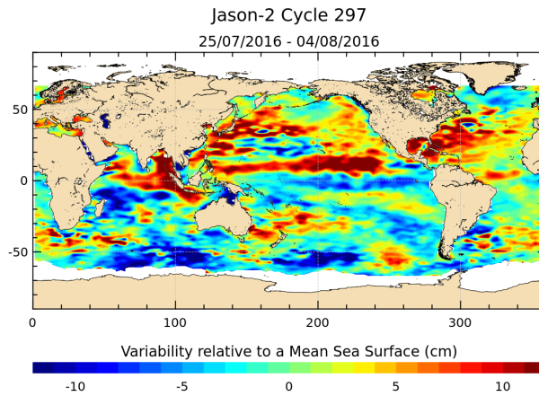
FIGURE 17 – Sea level anomaly relative to MSS for cycle 297.
