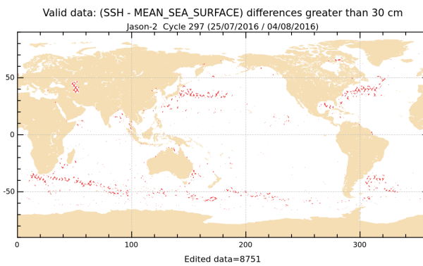
FIGURE 18 – Differences higher than a 30 cm threshold for cycle 297.
