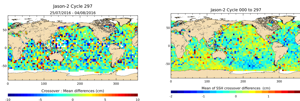
FIGURE 12 – Mean SSH at crossovers for cycle 297 (left) and over the whole Jason-2 period (right).
