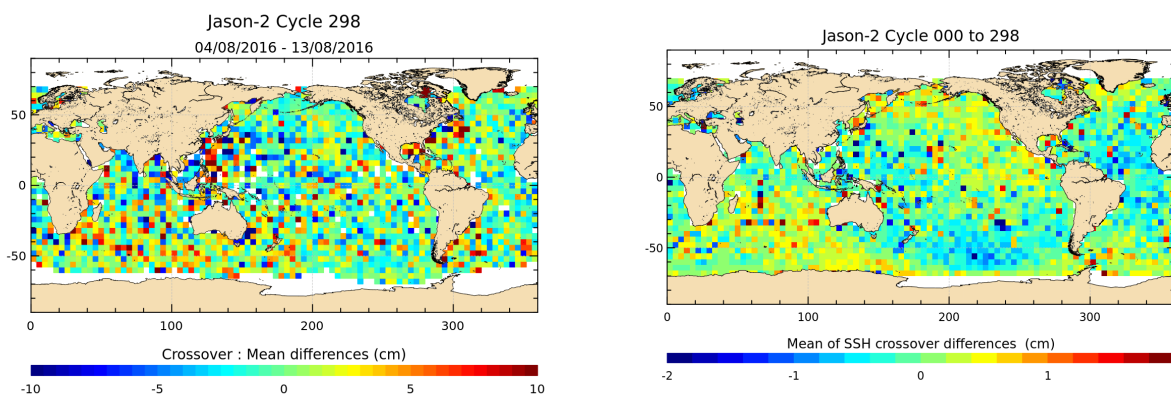
FIGURE 12 – Mean SSH at crossovers for cycle 298 (left) and over the whole Jason-2 period (right).
