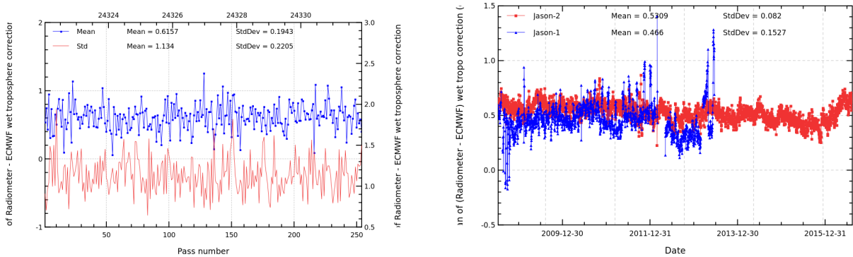
FIGURE 11 – Pass monitoring of wet troposphere differences between radiometer and ECMWF model for Jason-2 cycle 298 (left) and daily monitoring of wet troposphere differences between radiometer and ECMWF model (right).
