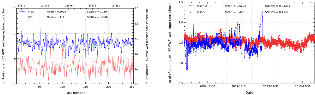
FIGURE 11 – Pass monitoring of wet troposphere differences between radiometer and ECMWF model for Jason-2 cycle 303 (left) and daily monitoring of wet troposphere differences between radiometer and ECMWF model (right).
