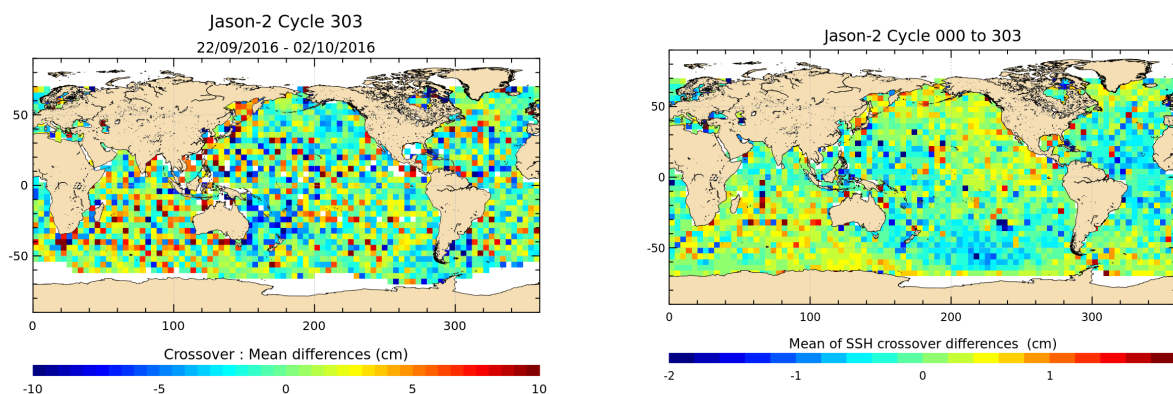
FIGURE 12 – Mean SSH at crossovers for cycle 303 (left) and over the whole Jason-2 period (right).
