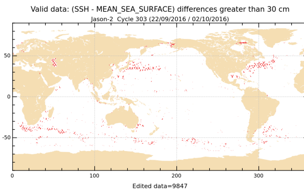
FIGURE 18 – Differences higher than a 30 cm threshold for cycle 303.
