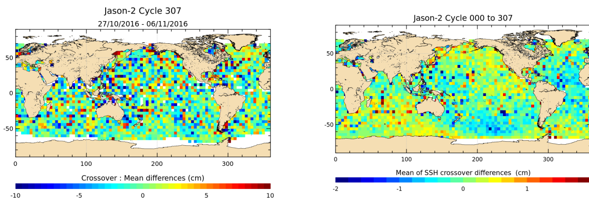
FIGURE 12 – Mean SSH at crossovers for cycle 307 (left) and over the whole Jason-2 period (right).
