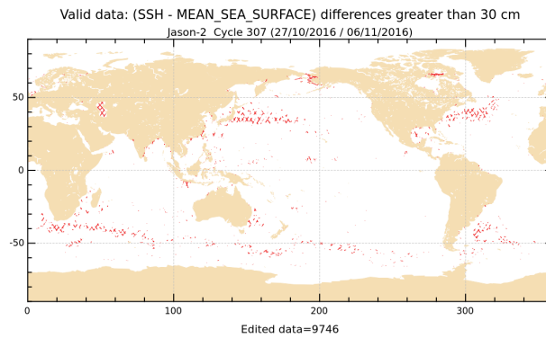
FIGURE 18 – Differences higher than a 30 cm threshold for cycle 307.
