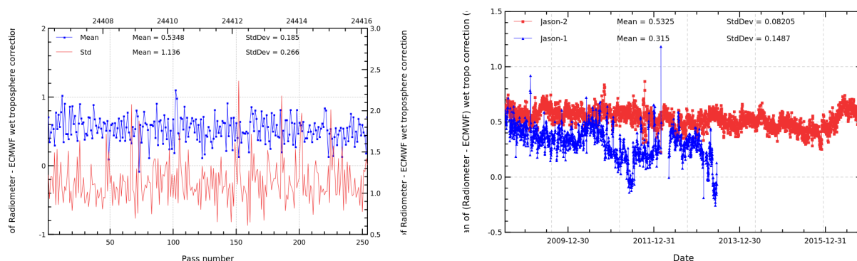
FIGURE 11 – Pass monitoring of wet troposphere differences between radiometer and ECMWF model for Jason-2 cycle 307 (left) and daily monitoring of wet troposphere differences between radiometer and ECMWF model (right).
