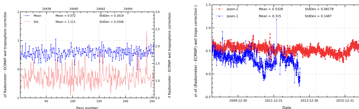
FIGURE 11 – Pass monitoring of wet troposphere differences between radiometer and ECMWF model for Jason-2 cycle 310 (left) and daily monitoring of wet troposphere differences between radiometer and ECMWF model (right).
