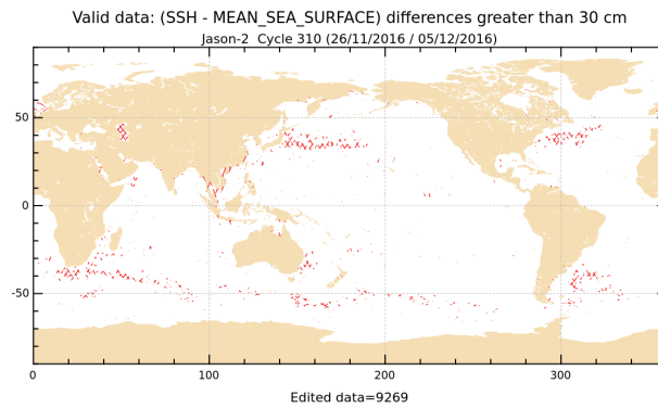
FIGURE 18 – Differences higher than a 30 cm threshold for cycle 310.
