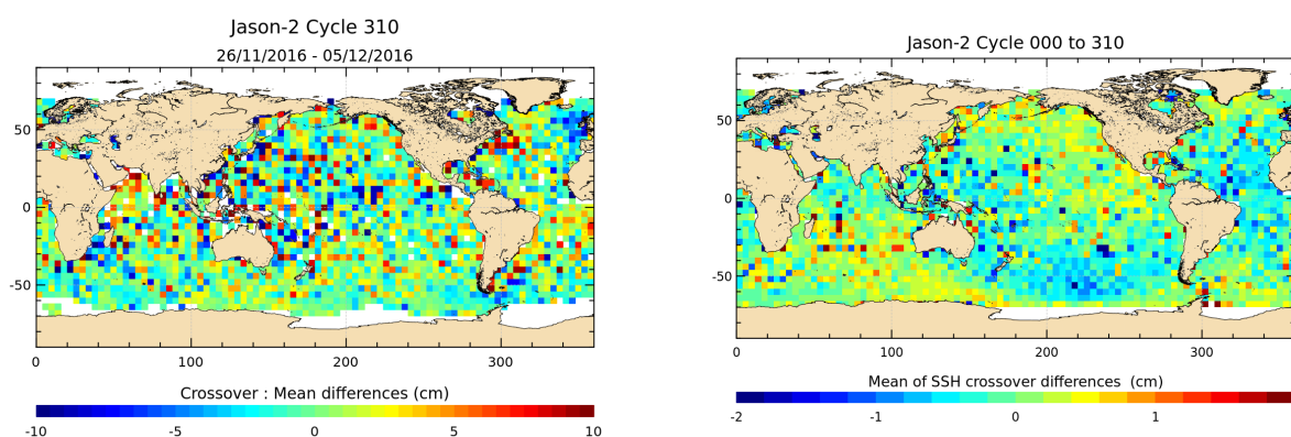
FIGURE 12 – Mean SSH at crossovers for cycle 310 (left) and over the whole Jason-2 period (right).
