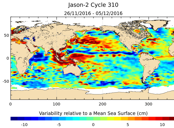
FIGURE 17 – Sea level anomaly relative to MSS for cycle 310.
