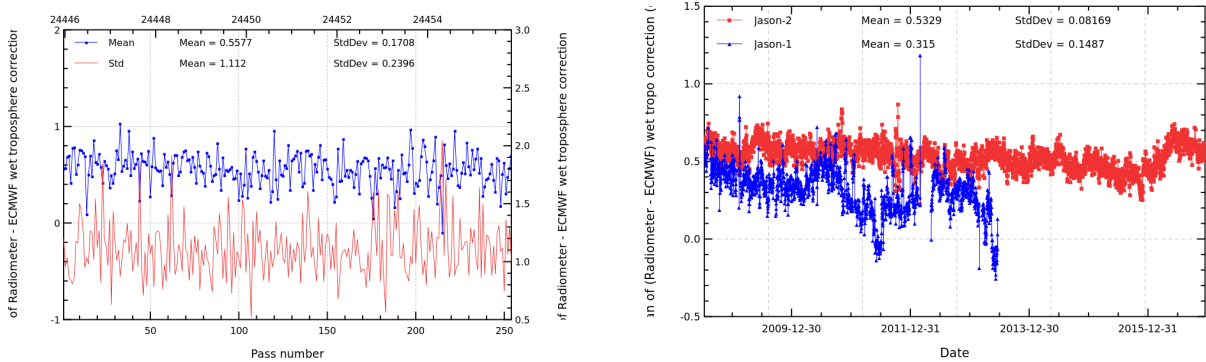
FIGURE 11 – Pass monitoring of wet troposphere differences between radiometer and ECMWF model for Jason-2 cycle 311 (left) and daily monitoring of wet troposphere differences between radiometer and ECMWF model (right).
