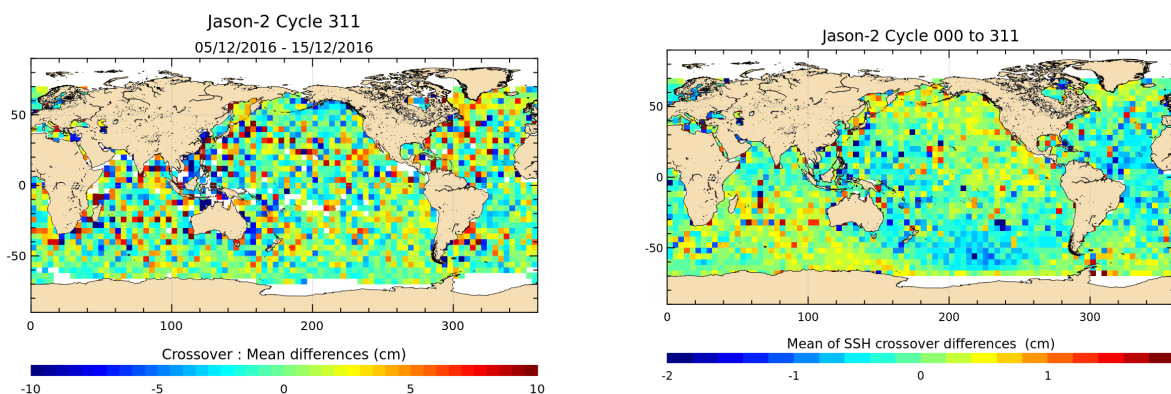
FIGURE 12 – Mean SSH at crossovers for cycle 311 (left) and over the whole Jason-2 period (right).
