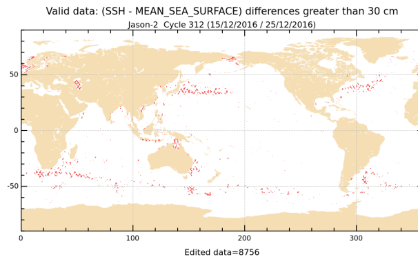
FIGURE 18 – Differences higher than a 30 cm threshold for cycle 312.
