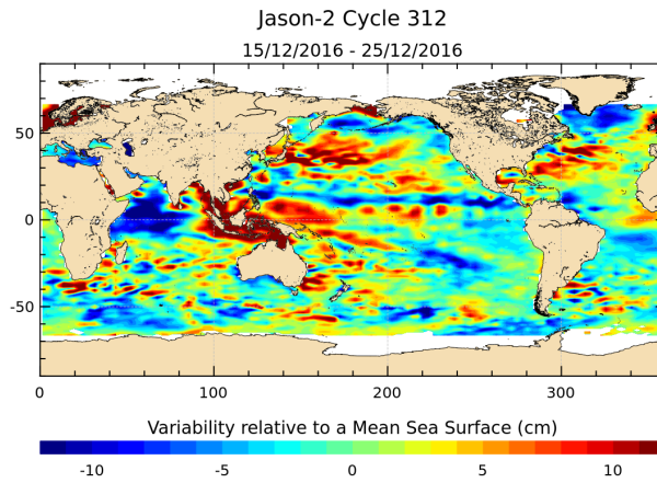
FIGURE 17 – Sea level anomaly relative to MSS for cycle 312.
