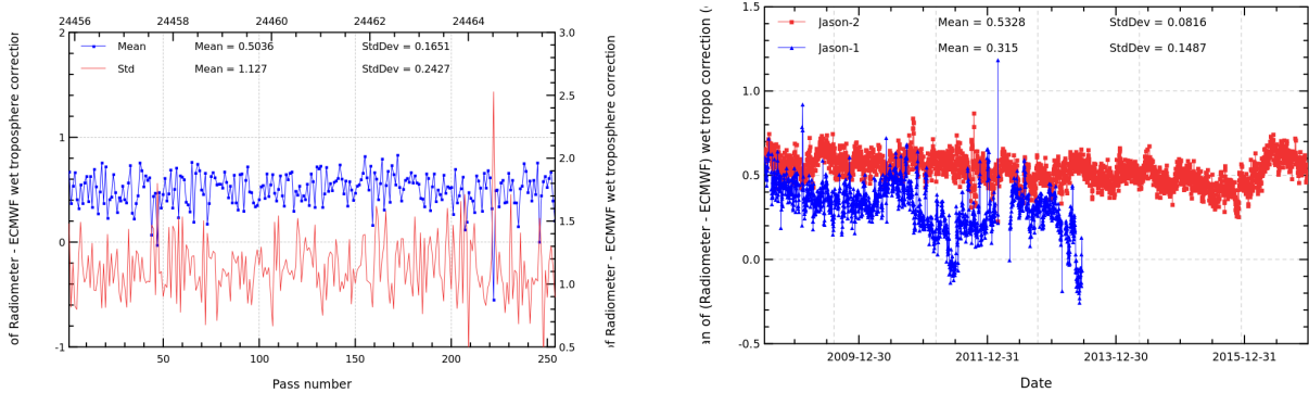
FIGURE 11 – Pass monitoring of wet troposphere differences between radiometer and ECMWF model for Jason-2 cycle 312 (left) and daily monitoring of wet troposphere differences between radiometer and ECMWF model (right).
