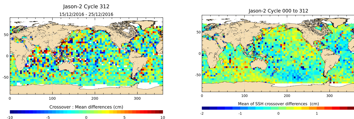
FIGURE 12 – Mean SSH at crossovers for cycle 312 (left) and over the whole Jason-2 period (right).
