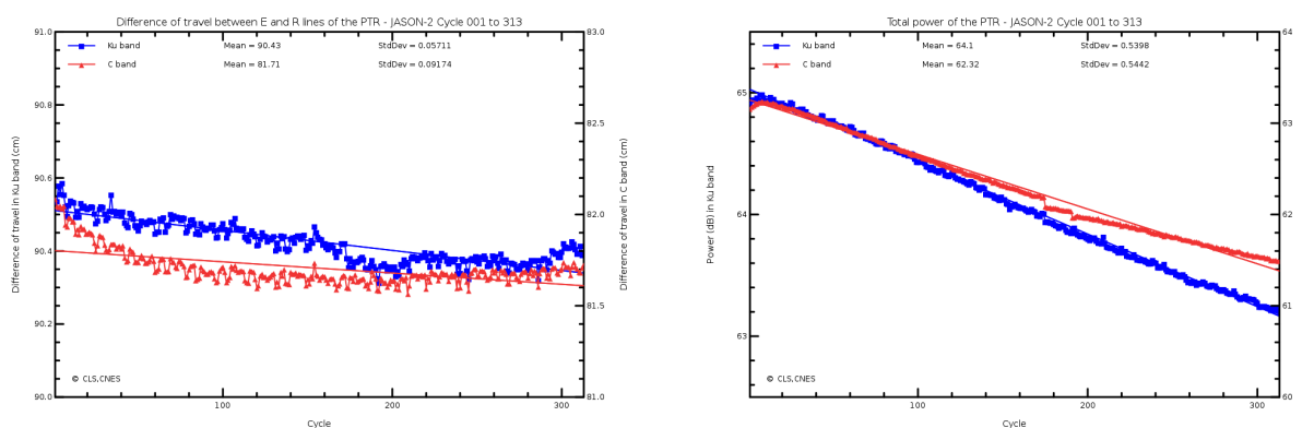
FIGURE 6 – Internal path delay (left) and total power of the PTR (right) for Ku- and C-band.
