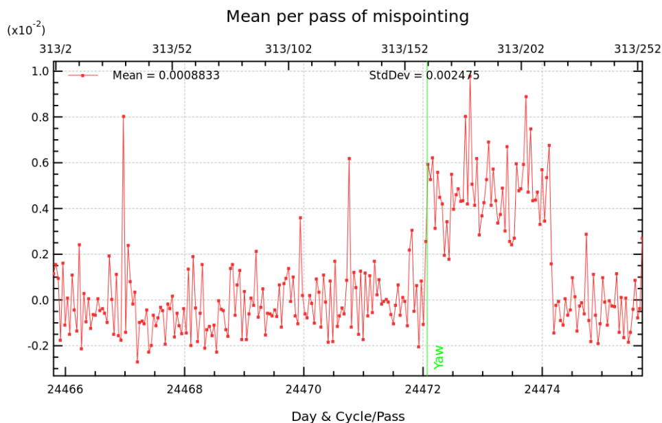
FIGURE 4 – Apparent squared mispointing from waveforms for cycle 313.
