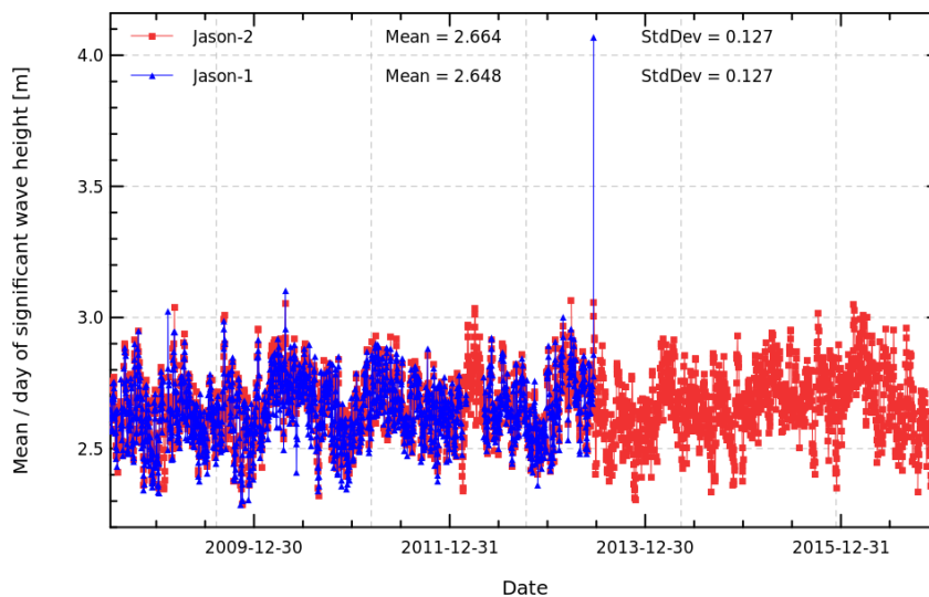
FIGURE 8 – Daily monitoring of Ku-band significant wave height for Jason-2 and Jason-1.
