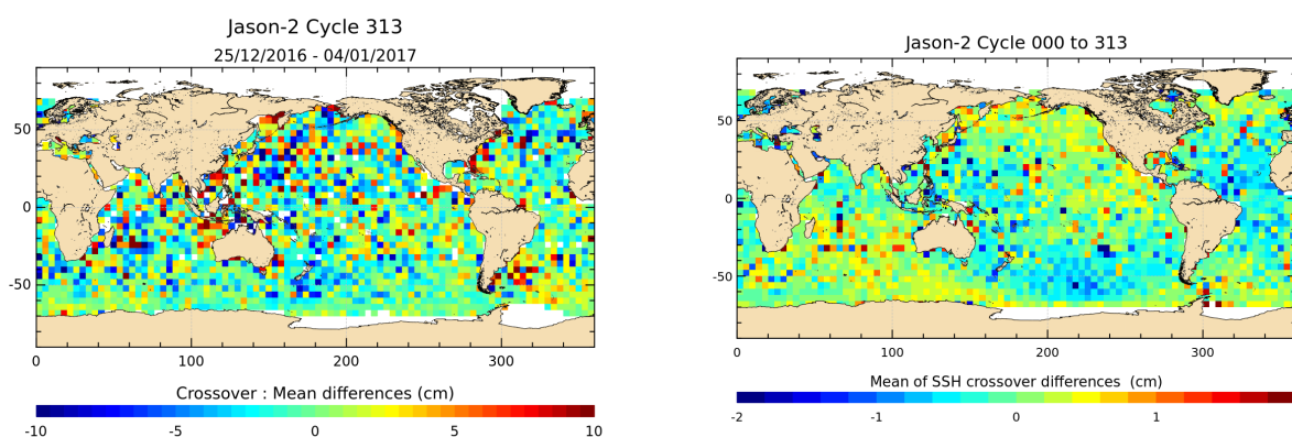
FIGURE 14 – Mean SSH at crossovers for cycle 313 (left) and over the whole Jason-2 period (right).
