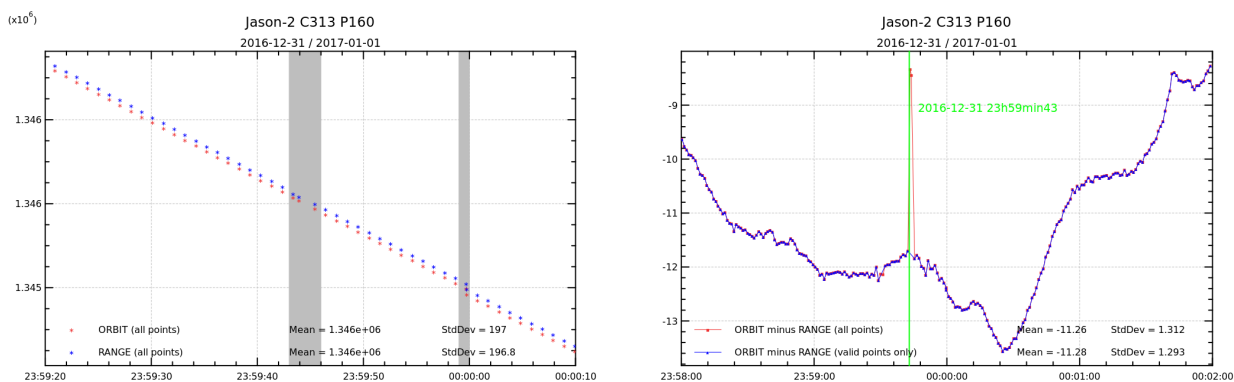
FIGURE 5 – Jason-2 along-track datation monitoring on cycle 313 pass 160. Datation points on orbit and range (left). Orbit minus range (right)
