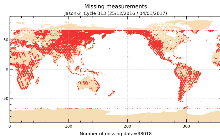
FIGURE 1 – Missing measurements for cycle 313.
