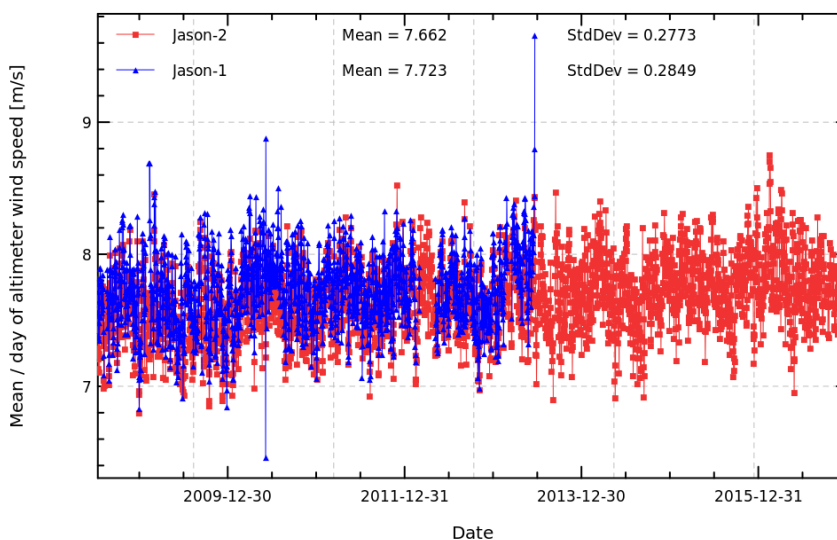
FIGURE 12 – Daily monitoring of altimeter wind speed for Jason-2 and Jason-1.
