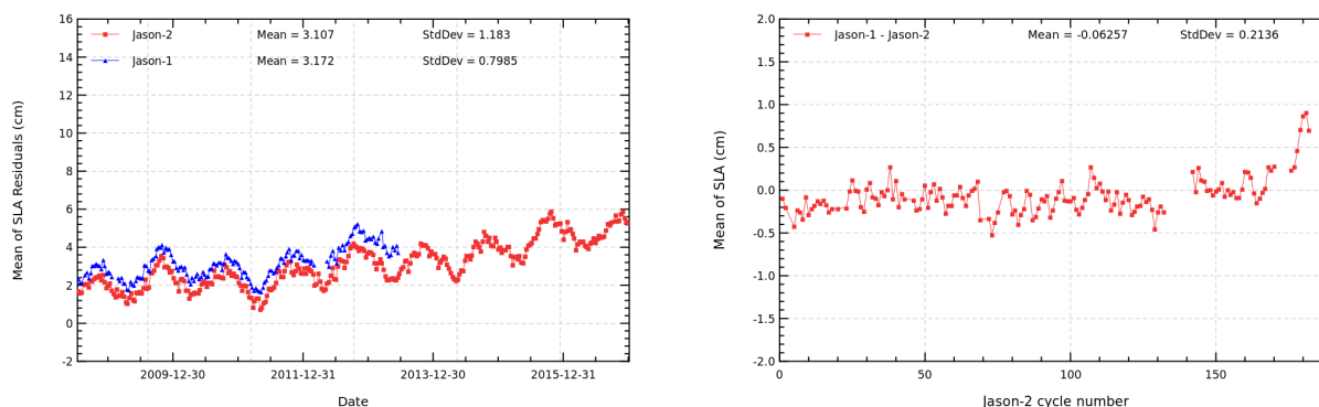
FIGURE 18 – Cyclic monitoring of mean SLA for Jason-1 and Jason-2 (left) and differences of (Jason-1 – Jason-2) mean SLA (right).
