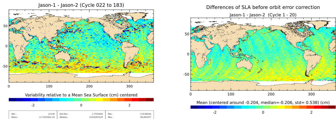
FIGURE 21 – Jason-1 – Jason-2 SLA differences averaged over Jason-2 period from cycle 022 until cycle 183 (left), and for tandem phase (cycle 001 to 020) (right).
