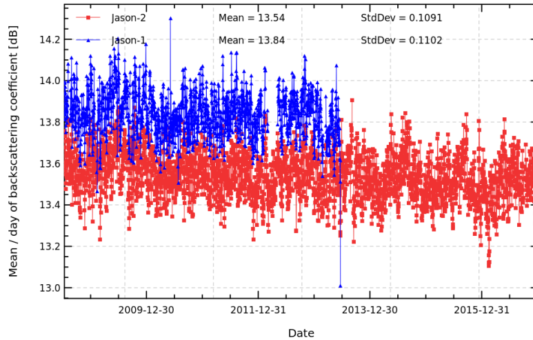
FIGURE 9 – Daily monitoring of Ku-band backscattering coefficient for Jason-2 and Jason-1.
