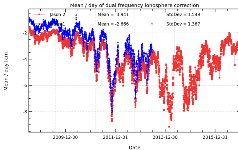
FIGURE 10 – Daily monitoring of dual-frequency ionosphere correction for Jason-2 and Jason-1.
