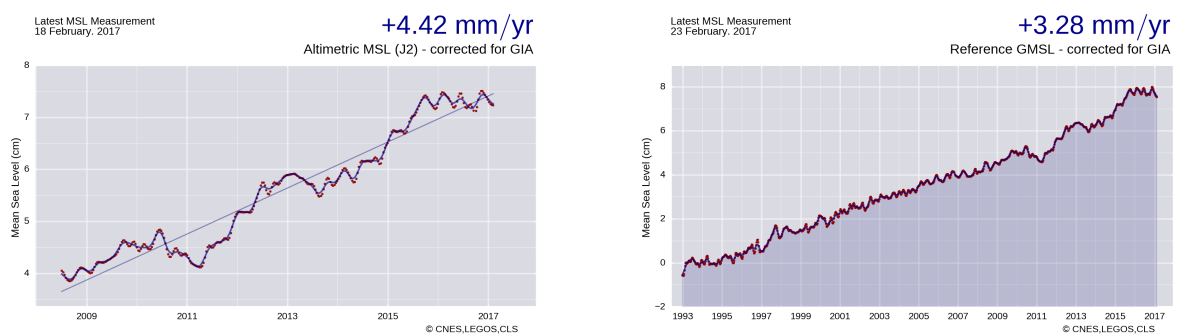
FIGURE 23 – Global MSL on Jason-2 mission (left) and with reference missions from 1993 onwards (right).
