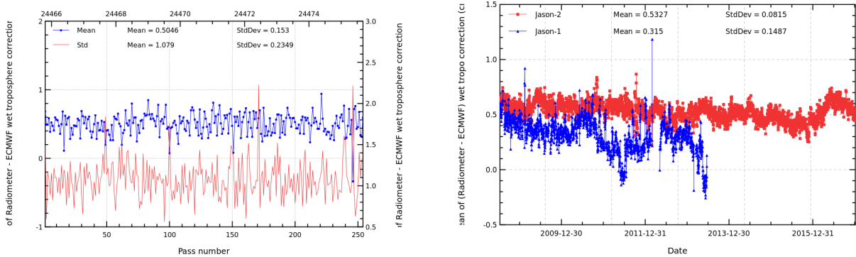
FIGURE 13 – Pass monitoring of wet troposphere differences between radiometer and ECMWF model for Jason-2 cycle 313 (left) and daily monitoring of wet troposphere differences between radiometer and ECMWF model (right).
